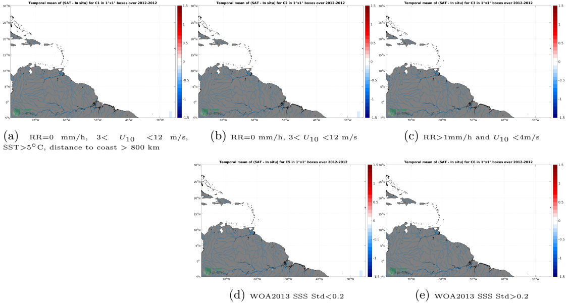
Figure 12: Temporal mean gridded over spatial boxes of size 1^{\circ}\times 1^{\circ} of \Delta\text{SSS} (Aquarius SSS L3 OR v5 - Monthly - Rain mask (NASA-GSFC) - TSG (Polarstern)) for 5 different subdatasets corresponding to:RR=0 mm/h, 3 < U_{10} < 12 m/s, SST >5^{\circ}\text{C} , distance to coast > 800 km (a), RR=0 mm/h, 3 < U_{10} < 12 m/s (b), RR >1 mm/h and U_{10} < 4 m/s (c), WOA2013 SSS Std <0.2 (d), WOA2013 SSS Std >0.2 (e).
