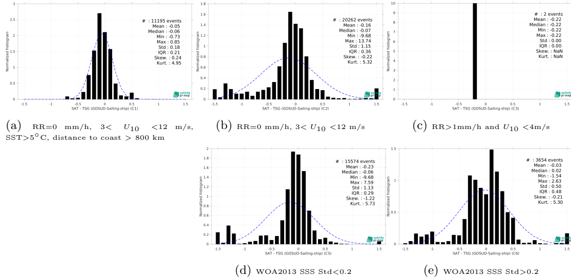
Figure 15: Normalized histogram of \Delta\text{SSS} (Aquarius SSS L3 OR v5 - Monthly - Rain mask (NASA-GSFC) - TSG (GOSUD-Sailing-ship)) for 5 different subdatasets corresponding to: RR=0 mm/h, 3 < U_{10} < 12 m/s, SST>5°C, distance to coast > 800 km (a), RR=0 mm/h, 3 < U_{10} < 12 m/s (b), RR>1mm/h and U_{10} < 4 m/s (c), WOA2013 SSS Std<0.2 (d), WOA2013 SSS Std>0.2 (e).
