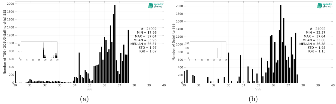
Figure 3: Histograms of SSS from TSG (GOSUD-Sailing-ship) (a) and Aquarius SSS L3 OR v5 - Monthly - Rain mask (NASA-GSFC) (b) considering all match-up pairs per bins of 0.1 over the Amazon and Orinoco river plumes Pi-MEP region and for the full satellite product period.
