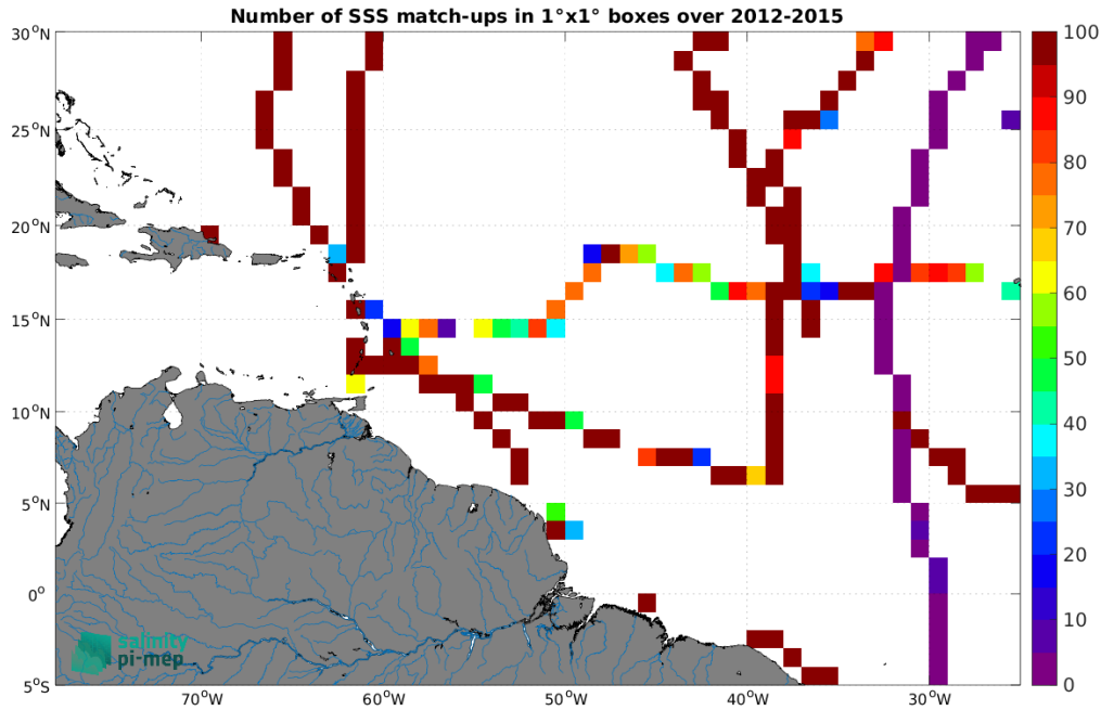
Figure 5: Number of SSS match-ups between TSG (GOSUD-Sailing-ship) SSS and the Aquarius SSS L3 OR v5 - Monthly - Rain mask (NASA-GSFC) SSS product for the Amazon and Orinoco river plumes Pi-MEP region over 1^\circ \times 1^\circ boxes and for the full satellite product period.
