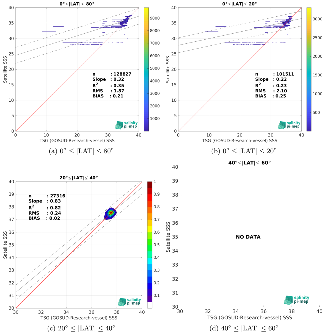
Figure 10: Contour maps of the concentration of Aquarius SSS L3 OR v5 - Monthly - Rain mask (NASA-GSFC) SSS (y-axis) versus TSG (GOSUD-Research-vessel) SSS (x-axis) at match-up pairs for different latitude bands. For each plot, the red line shows x=y . The black thin and dashed lines indicate a linear fit through the data cloud and the \pm 95\% confidence levels, respectively. The number match-up pairs n , the slope and R^2 coefficient of the linear fit, the root mean square (RMS) and the mean bias between satellite and in situ data are indicated for each latitude band in each plots.
