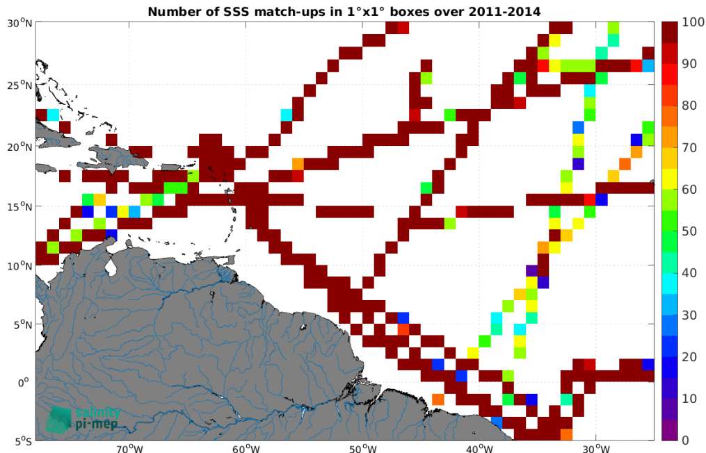
Figure 5: Number of SSS match-ups between TSG (GOSUD-Research-vessel) SSS and the Aquarius SSS L3 OR v5 - Monthly - Rain mask (NASA-GSFC) SSS product for the Amazon and Orinoco river plumes Pi-MEP region over 1^\circ \times 1^\circ boxes and for the full satellite product period.
