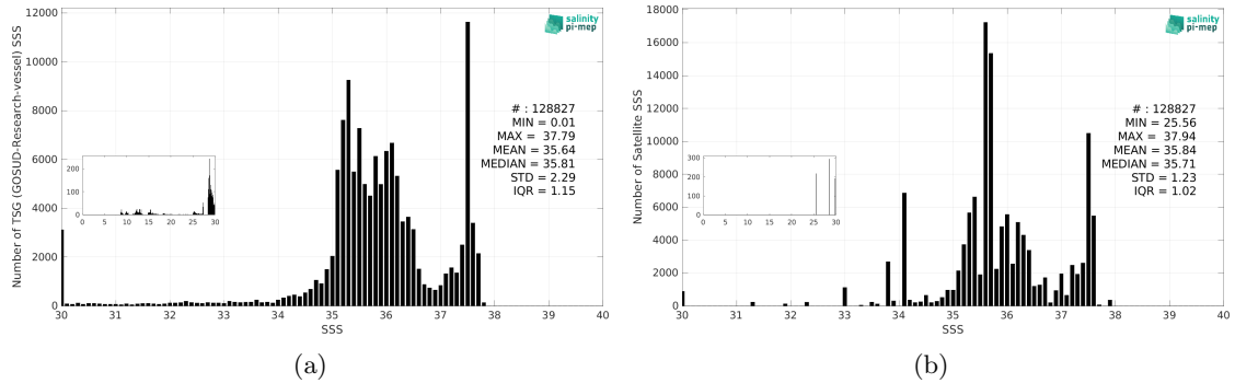
Figure 3: Histograms of SSS from TSG (GOSUD-Research-vessel) (a) and Aquarius SSS L3 OR v5 - Monthly - Rain mask (NASA-GSFC) (b) considering all match-up pairs per bins of 0.1 over the Amazon and Orinoco river plumes Pi-MEP region and for the full satellite product period.
