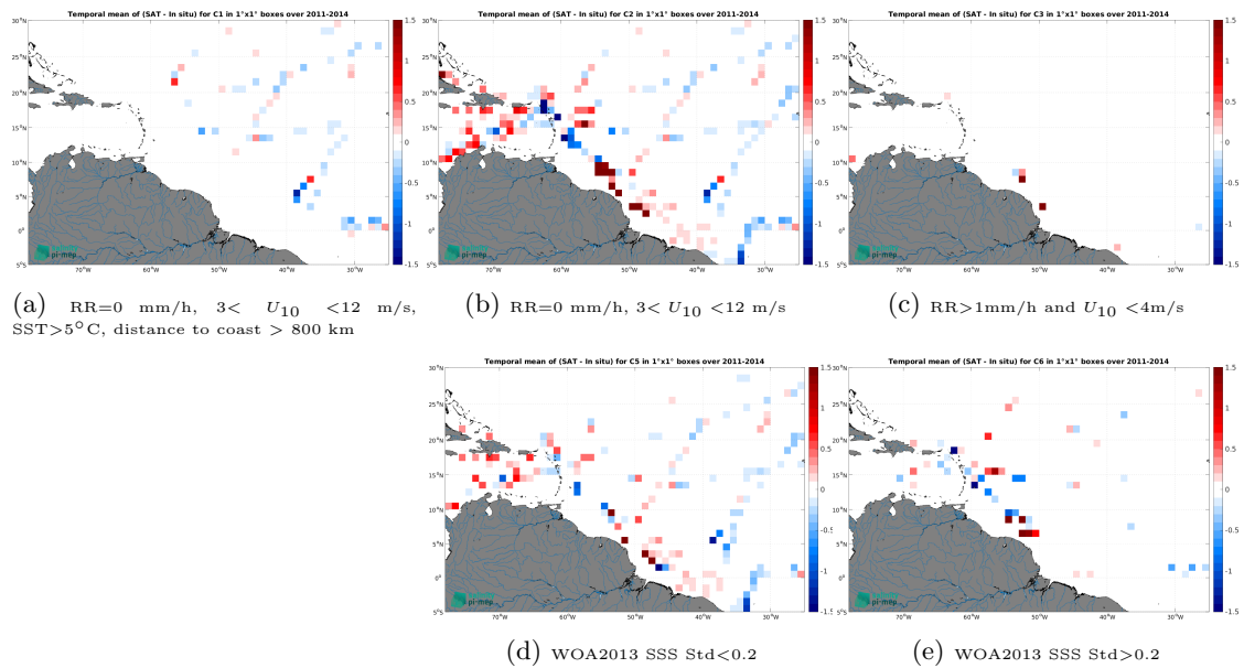
Figure 14: Temporal mean gridded over spatial boxes of size 1^\circ \times 1^\circ of \Delta SSS (Aquarius SSS L3 OR v5 - Monthly - Rain mask (NASA-GSFC) - TSG (GOSUD-Research-vessel)) for 5 different subdatasets corresponding to:RR=0 mm/h, 3 < U_{10} < 12 m/s, SST >5^\circ\text{C} , distance to coast > 800 km (a), RR=0 mm/h, 3 < U_{10} < 12 m/s (b), RR >1 mm/h and U_{10} < 4 m/s (c), WOA2013 SSS Std <0.2 (d), WOA2013 SSS Std >0.2 (e).
