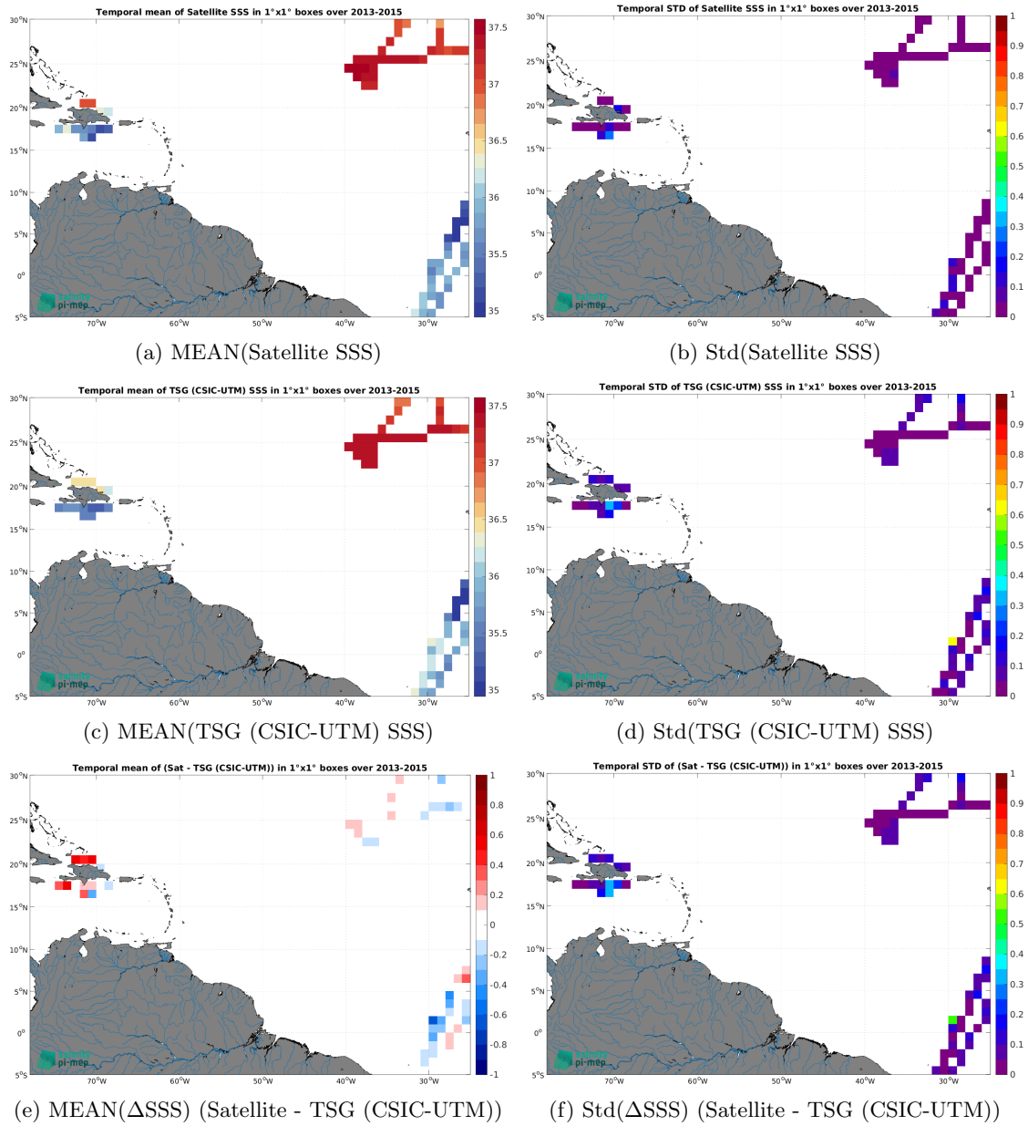
Figure 6: Temporal mean (left) and Std (right) of SSS from Aquarius SSS L3 OR v5 - Monthly - Rain mask (NASA-GSFC) (top), TSG (CSIC-UTM) (middle), and of \Delta SSS (Satellite - TSG (CSIC-UTM)). Only match-up pairs are used to generate these maps.
