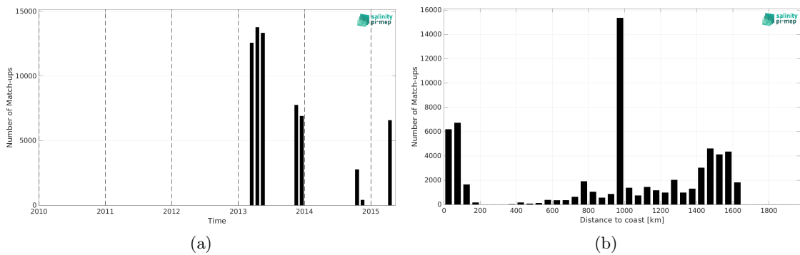
Figure 1: Number of match-ups between TSG (CSIC-UTM) and Aquarius SSS L3 OR v5 - Monthly - Rain mask (NASA-GSFC) SSS as a function of time (a) and as function of the distance to coast (b) over the Amazon and Orinoco river plumes Pi-MEP region and for the full satellite product period.
