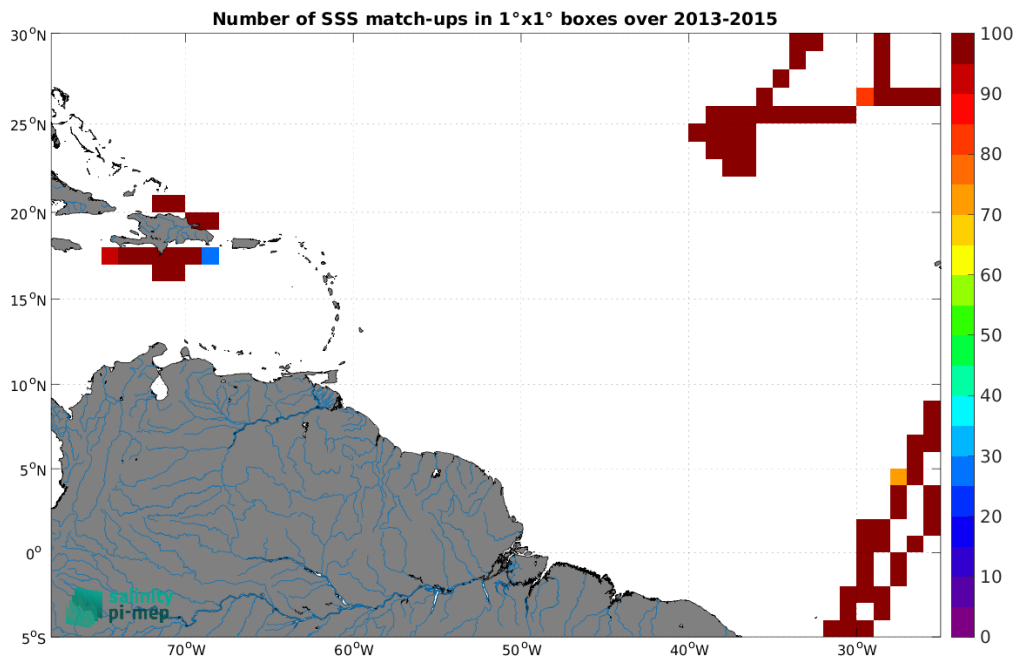
Figure 4: Number of SSS match-ups between TSG (CSIC-UTM) SSS and the Aquarius SSS L3 OR v5 - Monthly - Rain mask (NASA-GSFC) SSS product for the Amazon and Orinoco river plumes Pi-MEP region over 1^\circ \times 1^\circ boxes and for the full satellite product period.
