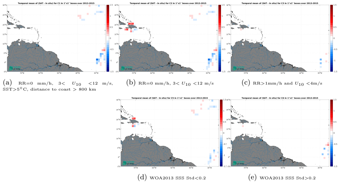
Figure 12: Temporal mean gridded over spatial boxes of size 1^{\circ}\times 1^{\circ} of \Delta\text{SSS} (Aquarius SSS L3 OR v5 - Monthly - Rain mask (NASA-GSFC) - TSG (CSIC-UTM)) for 5 different subdatasets corresponding to:RR=0 mm/h, 3 < U_{10} < 12 m/s, SST >5^{\circ}\text{C} , distance to coast > 800 km (a), RR=0 mm/h, 3 < U_{10} < 12 m/s (b), RR >1 mm/h and U_{10} < 4 m/s (c), WOA2013 SSS Std <0.2 (d), WOA2013 SSS Std >0.2 (e).
