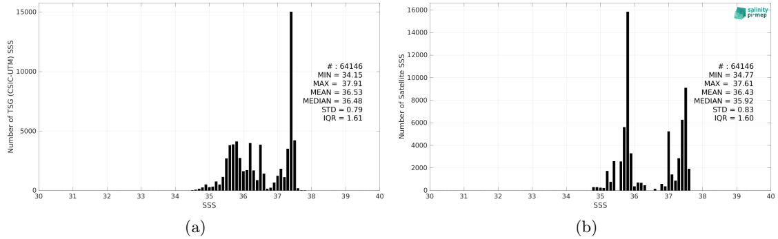
Figure 2: Histograms of SSS from TSG (CSIC-UTM) (a) and Aquarius SSS L3 OR v5 - Monthly - Rain mask (NASA-GSFC) (b) considering all match-up pairs per bins of 0.1 over the Amazon and Orinoco river plumes Pi-MEP region and for the full satellite product period.
