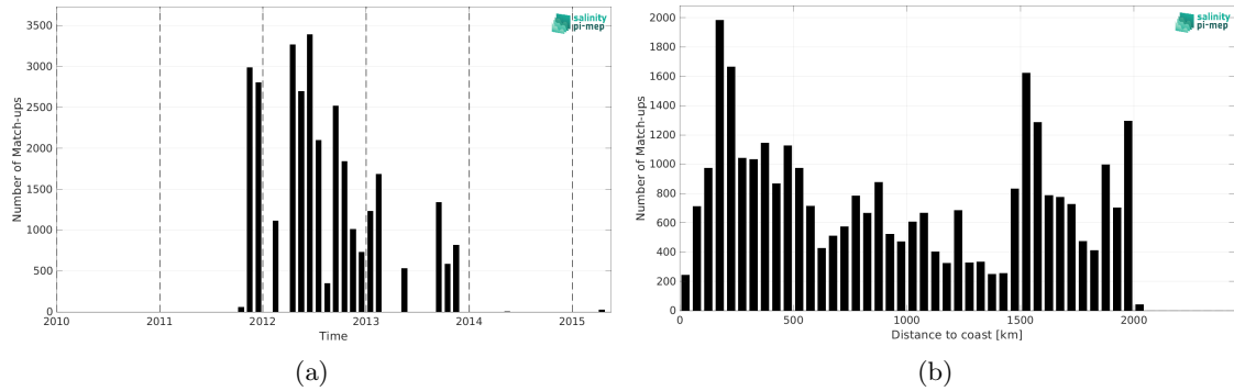
Figure 1: Number of match-ups between TSG (SAMOS) and Aquarius SSS L3 CAP v5 - 7-Day running (JPL) SSS as a function of time (a) and as function of the distance to coast (b) over the Amazon and Orinoco river plumes Pi-MEP region and for the full satellite product period.
