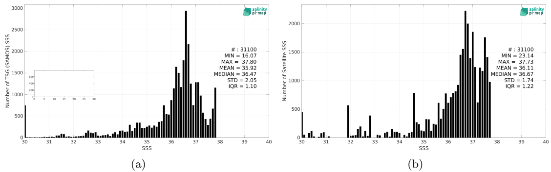
Figure 2: Histograms of SSS from TSG (SAMOS) (a) and Aquarius SSS L3 CAP v5 - 7-Day running (JPL) (b) considering all match-up pairs per bins of 0.1 over the Amazon and Orinoco river plumes Pi-MEP region and for the full satellite product period.
