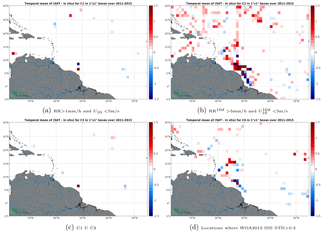
Figure 12: Temporal mean gridded over spatial boxes of size 1^\circ \times 1^\circ of \Delta SSS (Aquarius-L3-JPL-V5-7DAY-RUNNING - TSG-SAMOS) for 4 different subdatasets corresponding to: RR > 1mm/h and U_{10} < 5\text{m/s} (a), RR^{10d} > 5\text{mm/h} and U_{10}^{10d} < 5\text{m/s} (b), C1 U C2 (c), Locations where WOA2013 SSS STD > 0.2 (d).
