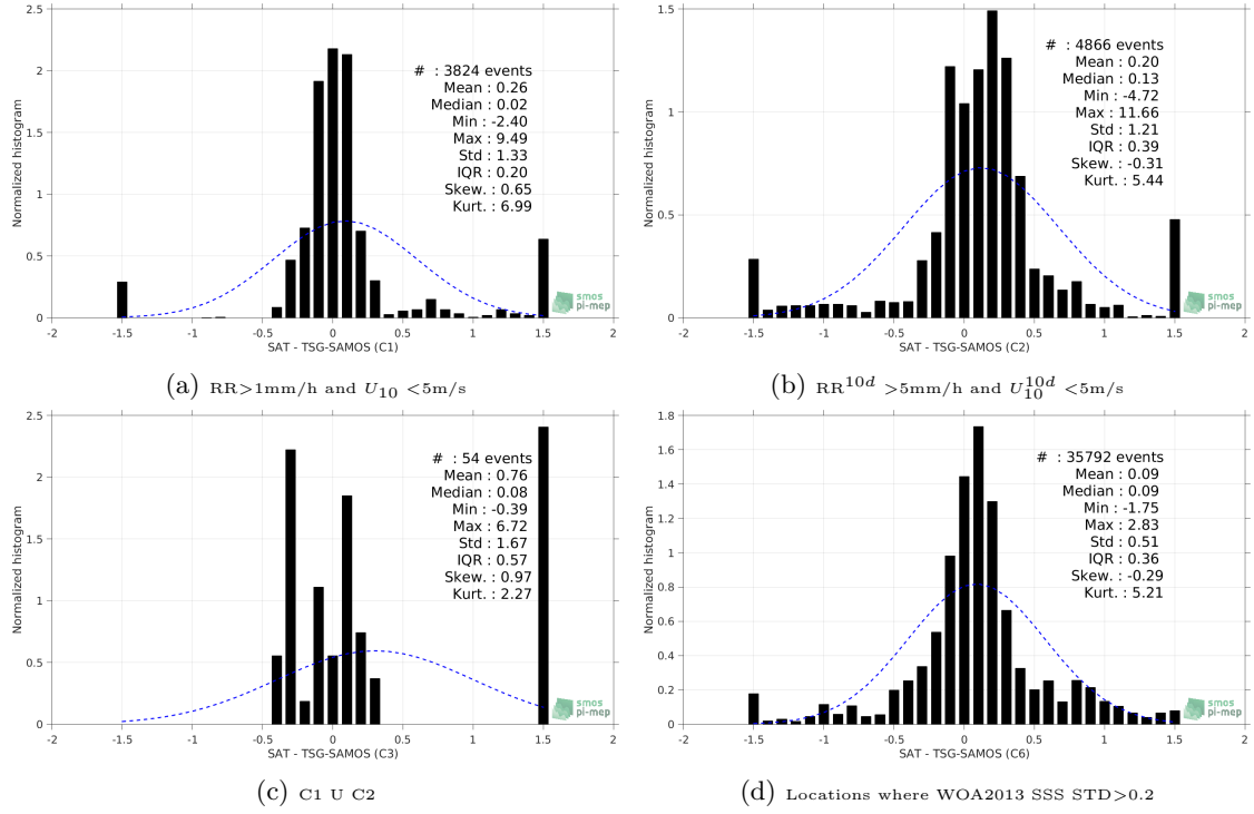
Figure 13: Normalized histogram of \Delta SSS (Aquarius-L3-JPL-V5-7DAY-RUNNING - TSG-SAMOS) for 6 different subdatasets corresponding to: RR > 1mm/h and U_{10} < 5 m/s (a), RR^{10d} > 5 mm/h and U_{10}^{10d} < 5 m/s (b), C1 U C2 (c), Locations where WOA2013 SSS STD > 0.2 (d).
