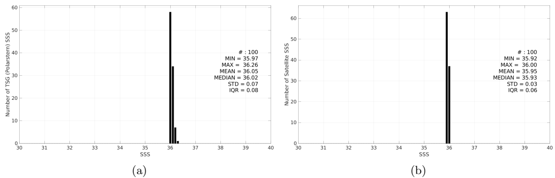
Figure 3: Histograms of SSS from TSG (Polarstern) (a) and Aquarius SSS L3 CAP v5 - 7-Day running (JPL) (b) considering all match-up pairs per bins of 0.1 over the Amazon and Orinoco river plumes Pi-MEP region and for the full satellite product period.
