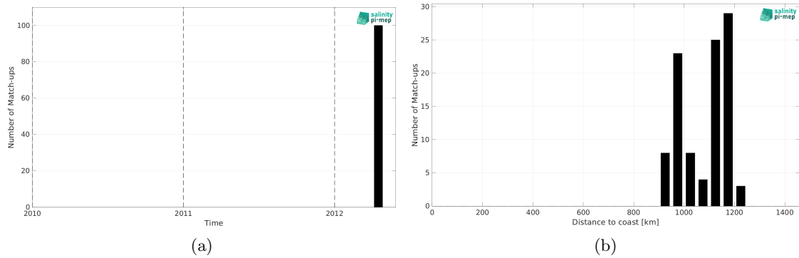
Figure 2: Number of match-ups between TSG (Polarstern) and Aquarius SSS L3 CAP v5 - 7-Day running (JPL) SSS as a function of time (a) and as function of the distance to coast (b) over the Amazon and Orinoco river plumes Pi-MEP region and for the full satellite product period.
