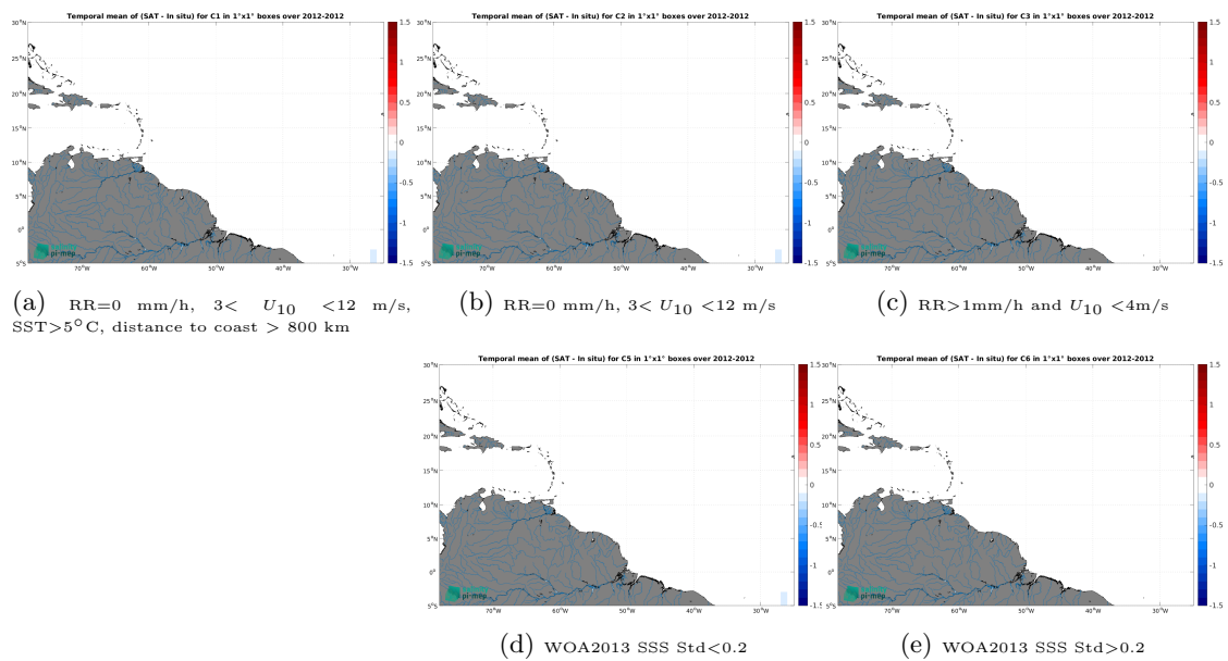
Figure 14: Temporal mean gridded over spatial boxes of size 1^\circ \times 1^\circ of \Delta SSS (Aquarius SSS L3 CAP v5 - 7-Day running (JPL) - TSG (Polarstern)) for 5 different subdatasets corresponding to:RR=0 mm/h, 3 < U_{10} < 12 m/s, SST >5^\circ C, distance to coast > 800 km (a), RR=0 mm/h, 3 < U_{10} < 12 m/s (b), RR >1 mm/h and U_{10} < 4 m/s (c), WOA2013 SSS Std <0.2 (d), WOA2013 SSS Std >0.2 (e).
