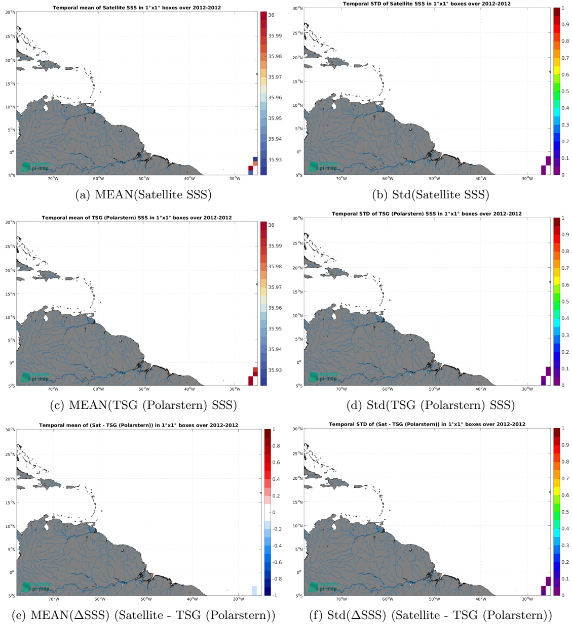
Figure 7: Temporal mean (left) and Std (right) of SSS from Aquarius SSS L3 CAP v5 - 7-Day running (JPL) (top), TSG (Polarstern) (middle), and of \Delta SSS (Satellite - TSG (Polarstern)). Only match-up pairs are used to generate these maps.
