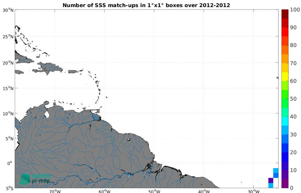
Figure 5: Number of SSS match-ups between TSG (Polarstern) SSS and the Aquarius SSS L3 CAP v5 - 7-Day running (JPL) SSS product for the Amazon and Orinoco river plumes Pi-MEP region over 1^\circ \times 1^\circ boxes and for the full satellite product period.
