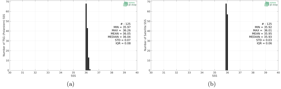
Figure 2: Histograms of SSS from TSG (Polarstern) (a) and Aquarius SSS L3 CAP v5 - 7-Day running (JPL) (b) considering all match-up pairs per bins of 0.1 over the Amazon and Orinoco river plumes Pi-MEP region and for the full satellite product period.
