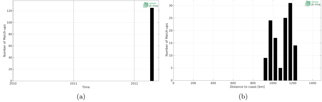
Figure 1: Number of match-ups between TSG (Polarstern) and Aquarius SSS L3 CAP v5 - 7-Day running (JPL) SSS as a function of time (a) and as function of the distance to coast (b) over the Amazon and Orinoco river plumes Pi-MEP region and for the full satellite product period.
