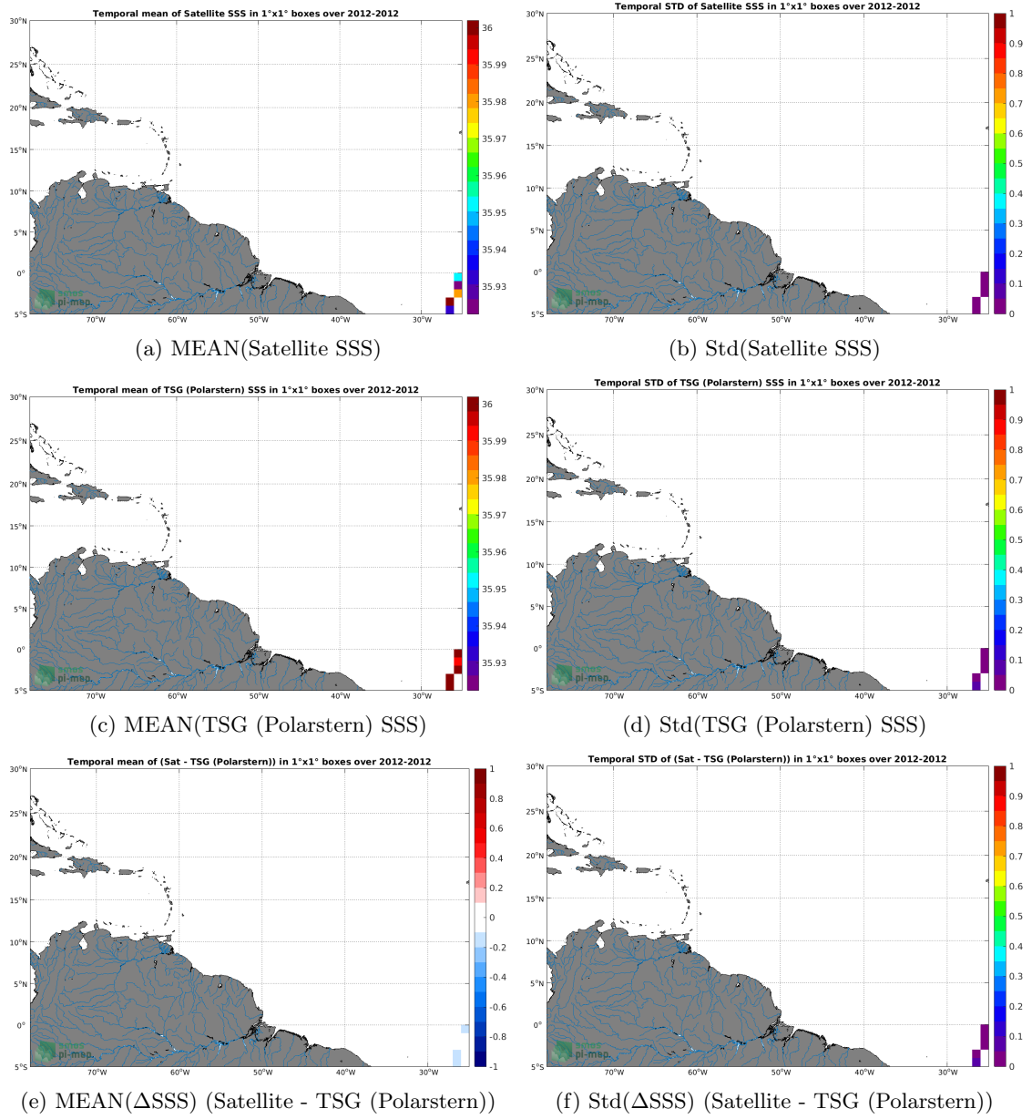
Figure 6: Temporal mean (left) and Std (right) of SSS from Aquarius SSS L3 CAP v5 - 7-Day running (JPL) (top), TSG (Polarstern) (middle), and of \Delta SSS (Satellite - TSG (Polarstern)). Only match-pairs are used to generate these maps.
