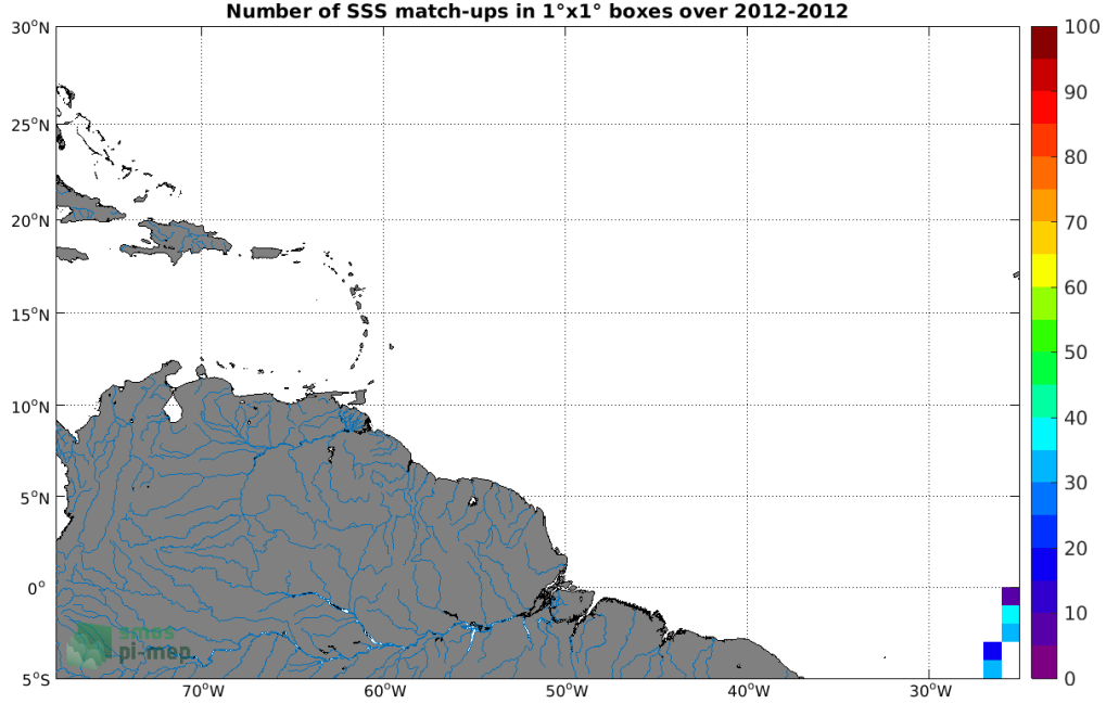
Figure 4: Number of SSS match-ups between TSG (Polarstern) SSS and the Aquarius SSS L3 CAP v5 - 7-Day running (JPL) SSS product for the Amazon and Orinoco river plumes Pi-MEP region over 1^\circ \times 1^\circ boxes and for the full satellite product period.
