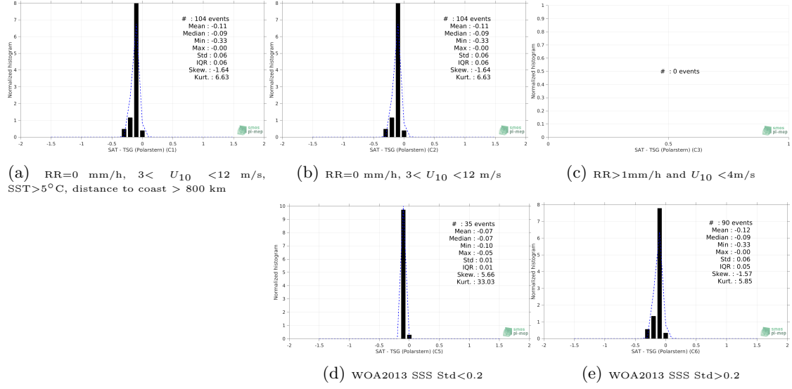
Figure 13: Normalized histogram of \Delta\text{SSS} (Aquarius SSS L3 CAP v5 - 7-Day running (JPL) - TSG (Polarstern)) for 5 different subdatasets corresponding to: \text{RR}=0 \text{ mm/h} , 3 < U_{10} < 12 \text{ m/s} , \text{SST} > 5^\circ\text{C} , distance to coast > 800 \text{ km} (a), \text{RR}=0 \text{ mm/h} , 3 < U_{10} < 12 \text{ m/s} (b), \text{RR} > 1 \text{ mm/h} and U_{10} < 4 \text{ m/s} (c), WOA2013 SSS Std < 0.2 (d), WOA2013 SSS Std > 0.2 (e).
