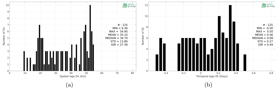
Figure 5: Histograms of the spatial (a) and temporal (b) lags between the time of the TSG-POLARSTERN measurements and the date of the corresponding Aquarius-L3-JPL-V5-7DAY-RUNNING SSS product.
