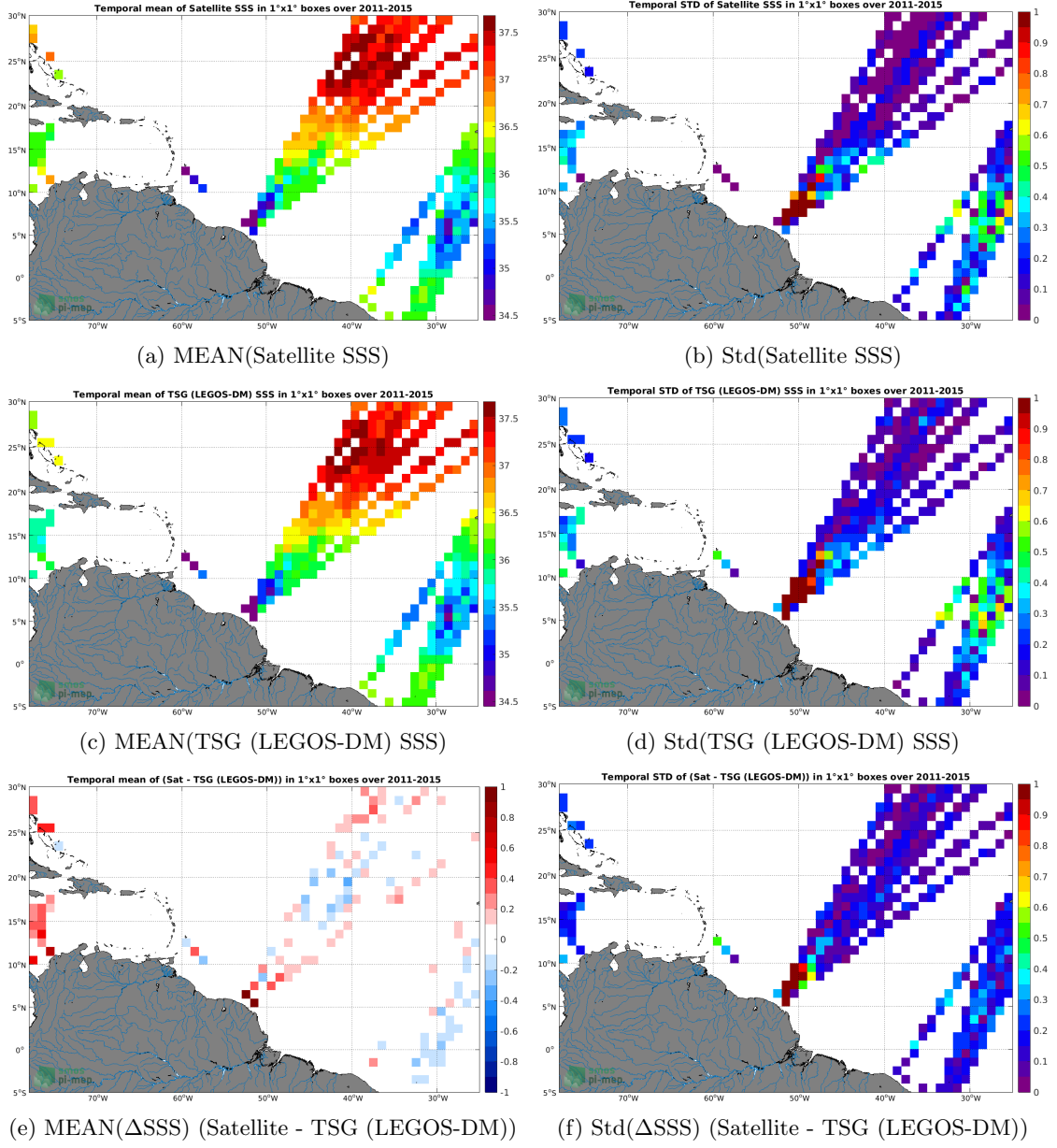
Figure 6: Temporal mean (left) and Std (right) of SSS from Aquarius SSS L3 CAP v5 - 7-Day running (JPL) (top), TSG (LEGOS-DM) (middle), and of \Delta SSS (Satellite - TSG (LEGOS-DM)). Only match-pairs are used to generate these maps.
