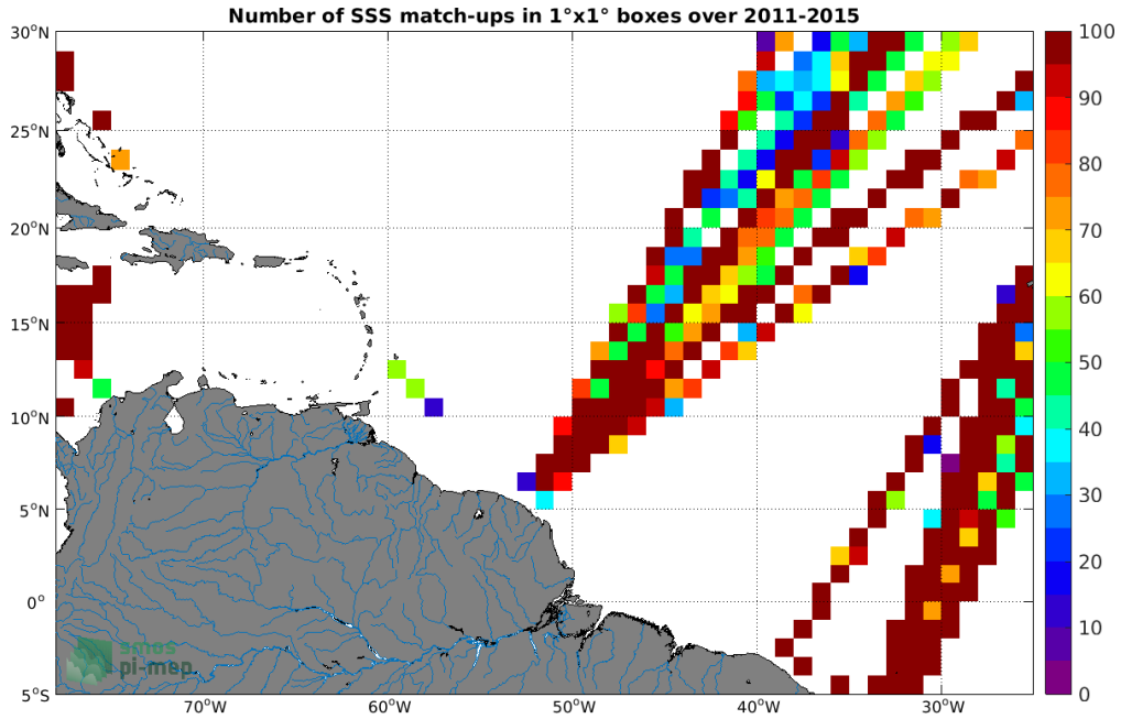
Figure 4: Number of SSS match-ups between TSG (LEGOS-DM) SSS and the Aquarius SSS L3 CAP v5 - 7-Day running (JPL) SSS product for the Amazon and Orinoco river plumes Pi-MEP region over 1°x1° boxes and for the full satellite product period.
