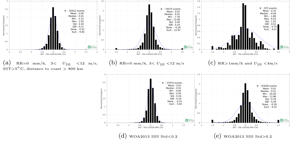
Figure 13: Normalized histogram of \Delta\text{SSS} (Aquarius SSS L3 CAP v5 - 7-Day running (JPL) - TSG (LEGOS-DM)) for 5 different subdatasets corresponding to: RR=0 mm/h, 3 < U_{10} < 12 m/s, SST>5°C, distance to coast > 800 km (a), RR=0 mm/h, 3 < U_{10} < 12 m/s (b), RR>1mm/h and U_{10} < 4 m/s (c), WOA2013 SSS Std<0.2 (d), WOA2013 SSS Std>0.2 (e).
