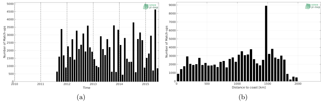
Figure 1: Number of match-ups between TSG-LEGOS-DM and Aquarius-L3-JPL-V5-7DAY-RUNNING SSS as a function of time (a) and as function of the distance to coast (b) over the Amazon and Orinoco river plumes Pi-MEP region and for the full satellite product period.
