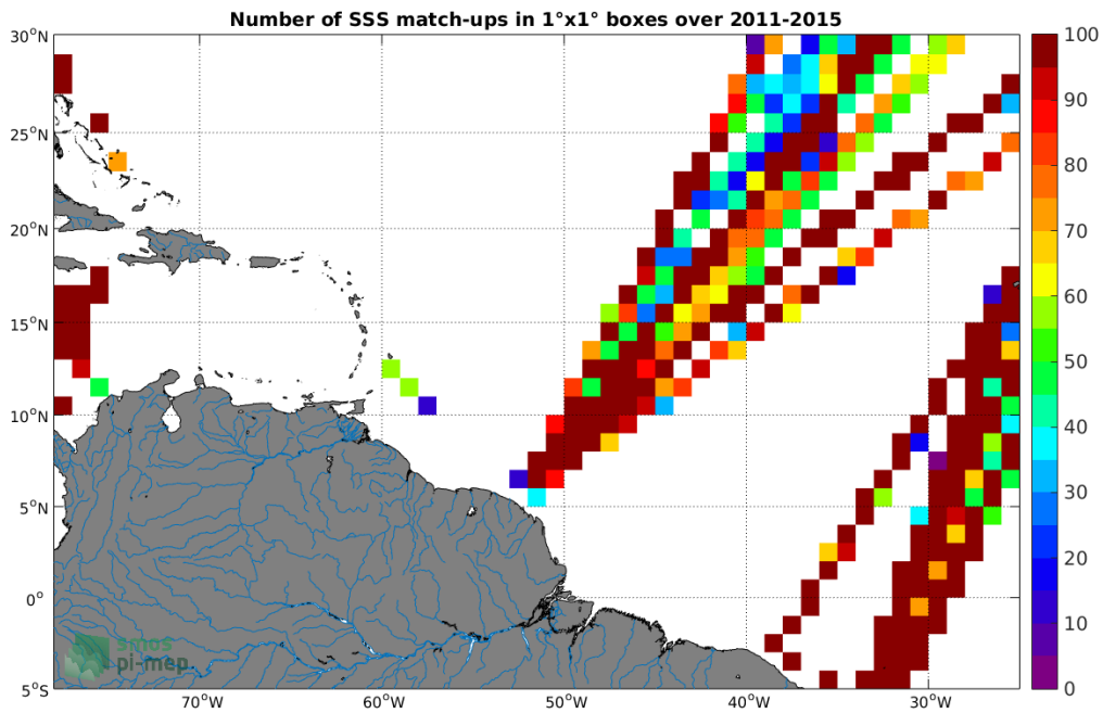
Figure 4: Number of SSS match-ups between TSG-LEGOS-DM SSS and the Aquarius-L3-JPL-V5-7DAY-RUNNING SSS product for the Amazon and Orinoco river plumes Pi-MEP region over 1^\circ \times 1^\circ boxes and for the full satellite product period.
