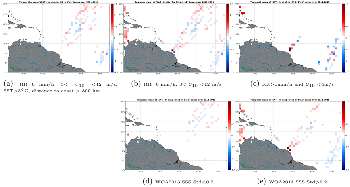
Figure 12: Temporal mean gridded over spatial boxes of size 1^\circ \times 1^\circ of \Delta SSS (Aquarius-L3-JPL-V5-7DAY-RUNNING - TSG-LEGOS-DM) for 5 different subdatasets corresponding to: RR=0 mm/h, 3 < U_{10} < 12 m/s, SST > 5^\circ C , distance to coast > 800 km (a), RR=0 mm/h, 3 < U_{10} < 12 m/s (b), RR > 1 mm/h and U_{10} < 4 m/s (c), WOA2013 SSS Std < 0.2 (d), WOA2013 SSS Std > 0.2 (e).
