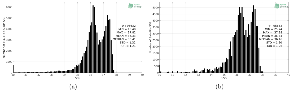
Figure 2: Histograms of SSS from TSG-LEGOS-DM (a) and Aquarius-L3-JPL-V5-7DAY-RUNNING (b) considering all match-up pairs per bins of 0.1 over the Amazon and Orinoco river plumes Pi-MEP region and for the full satellite product period.
