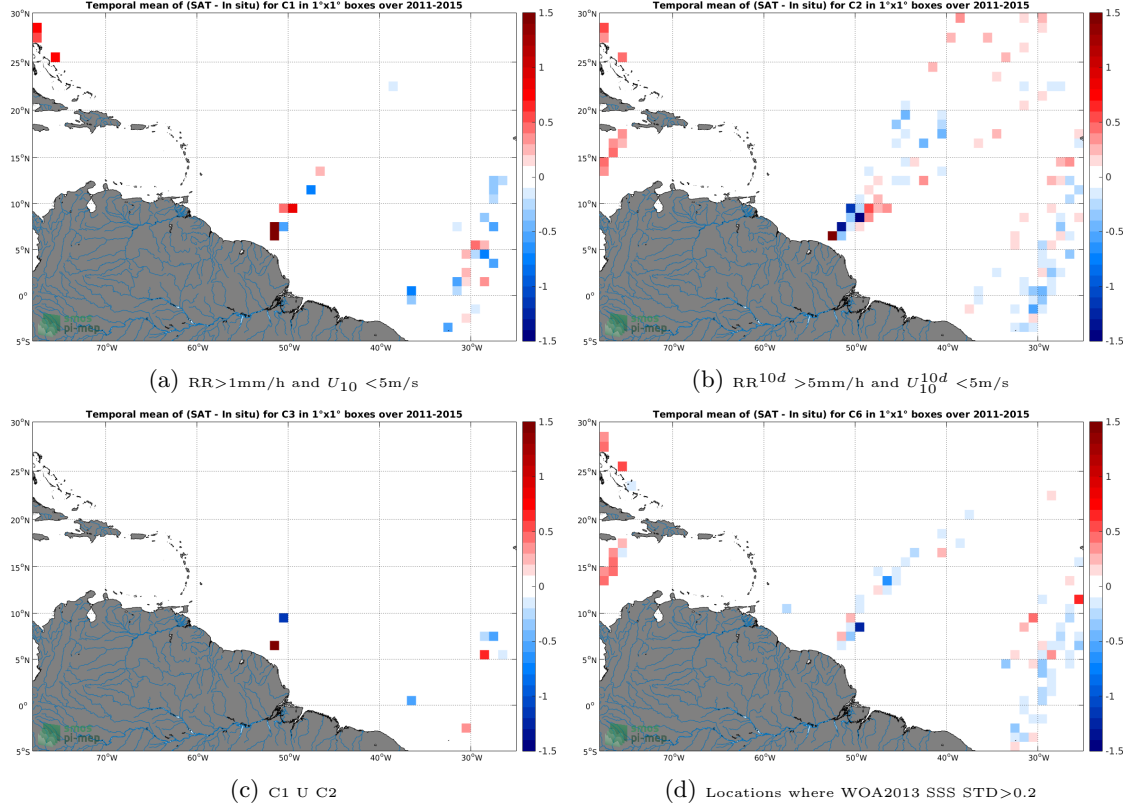
Figure 12: Temporal mean gridded over spatial boxes of size 1^\circ \times 1^\circ of \Delta SSS (Aquarius-L3-JPL-V5-7DAY-RUNNING - TSG-LEGOS-DM) for 4 different subdatasets corresponding to: RR > 1\text{mm/h} and U_{10} < 5\text{m/s} (a), RR^{10d} > 5\text{mm/h} and U_{10}^{10d} < 5\text{m/s} (b), C1 U C2 (c), Locations where WOA2013 SSS STD > 0.2 (d).
