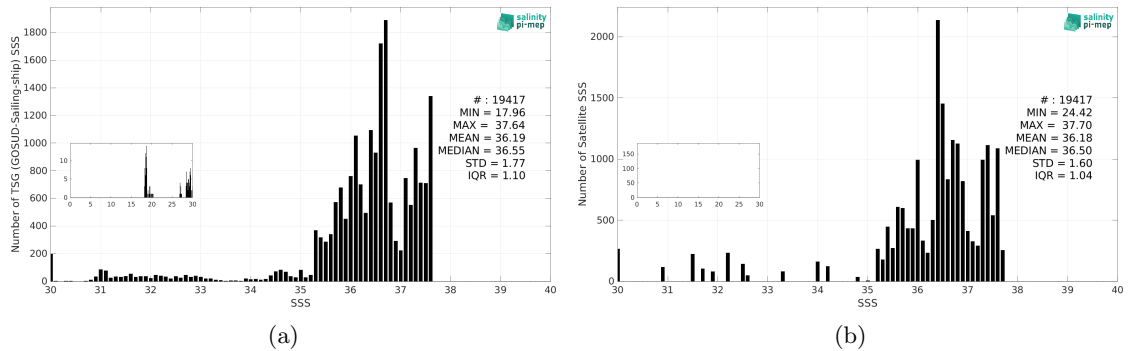
Figure 3: Histograms of SSS from TSG (GOSUD-Sailing-ship) (a) and Aquarius SSS L3 CAP v5 - 7-Day running (JPL) (b) considering all match-up pairs per bins of 0.1 over the Amazon and Orinoco river plumes Pi-MEP region and for the full satellite product period.
