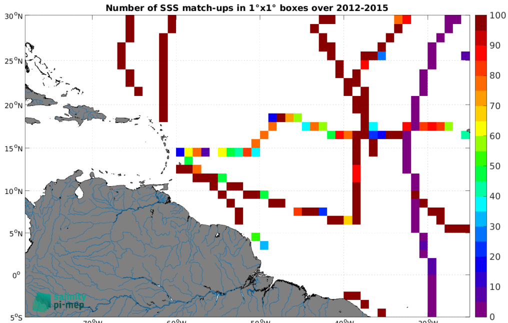
Figure 5: Number of SSS match-ups between TSG (GOSUD-Sailing-ship) SSS and the Aquarius SSS L3 CAP v5 - 7-Day running (JPL) SSS product for the Amazon and Orinoco river plumes Pi-MEP region over 1^\circ \times 1^\circ boxes and for the full satellite product period.
