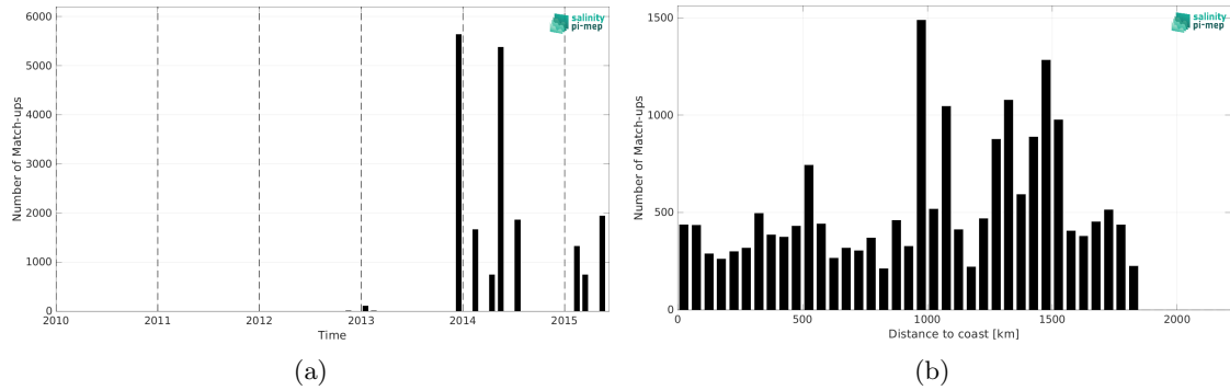
Figure 2: Number of match-ups between TSG (GOSUD-Sailing-ship) and Aquarius SSS L3 CAP v5 - 7-Day running (JPL) SSS as a function of time (a) and as function of the distance to coast (b) over the Amazon and Orinoco river plumes Pi-MEP region and for the full satellite product period.
