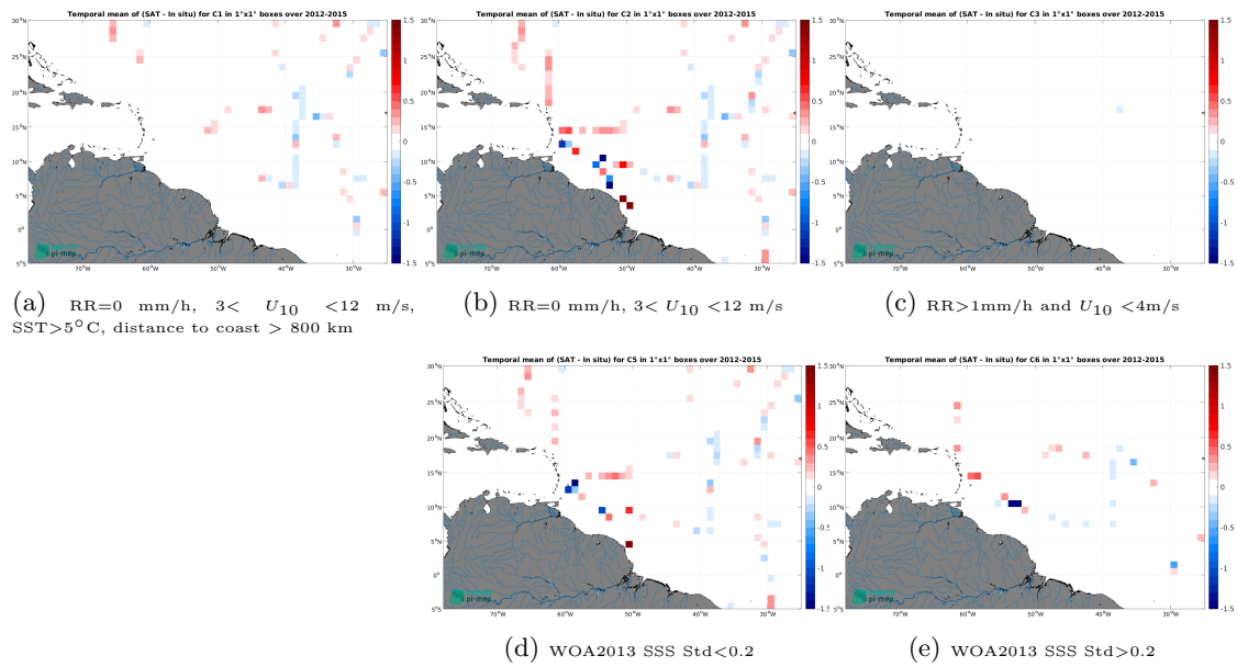
Figure 14: Temporal mean gridded over spatial boxes of size 1^\circ \times 1^\circ of \Delta\text{SSS} (Aquarius SSS L3 CAP v5 - 7-Day running (JPL) - TSG (GOSUD-Sailing-ship)) for 5 different subdatasets corresponding to:RR=0 mm/h, 3 < U_{10} < 12 m/s, SST >5^\circ\text{C} , distance to coast > 800 km (a), RR=0 mm/h, 3 < U_{10} < 12 m/s (b), RR >1 mm/h and U_{10} < 4 m/s (c), WOA2013 SSS Std <0.2 (d), WOA2013 SSS Std >0.2 (e).
