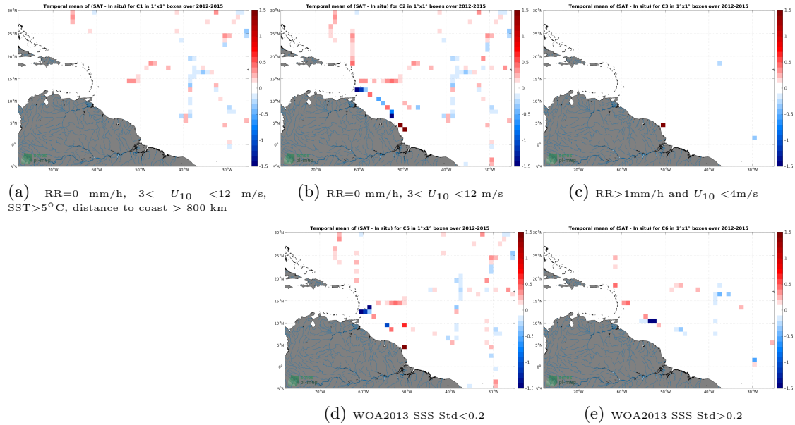
Figure 12: Temporal mean gridded over spatial boxes of size 1^{\circ}\times 1^{\circ} of \Delta SSS (Aquarius SSS L3 CAP v5 - 7-Day running (JPL) - TSG (GOSUD-Sailing-ship)) for 5 different subdatasets corresponding to:RR=0 mm/h, 3 < U_{10} < 12 m/s, SST >5^{\circ}\text{C} , distance to coast > 800 km (a), RR=0 mm/h, 3 < U_{10} < 12 m/s (b), RR >1 mm/h and U_{10} < 4 m/s (c), WOA2013 SSS Std <0.2 (d), WOA2013 SSS Std >0.2 (e).
