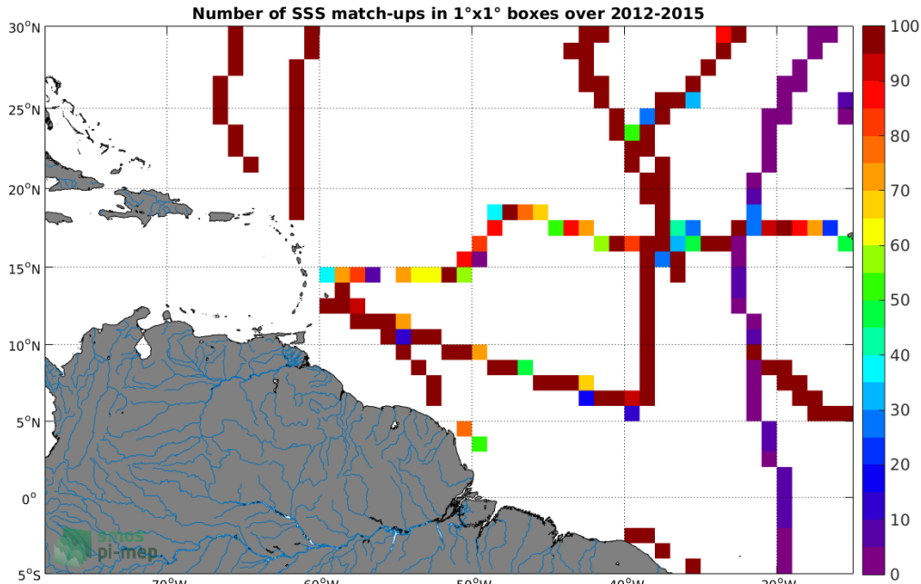
Figure 4: Number of SSS match-ups between TSG (GOSUD-Sailing-ship) SSS and the Aquarius SSS L3 CAP v5 - 7-Day running (JPL) SSS product for the Amazon and Orinoco river plumes Pi-MEP region over 1^{\circ} \times 1^{\circ} boxes and for the full satellite product period.
