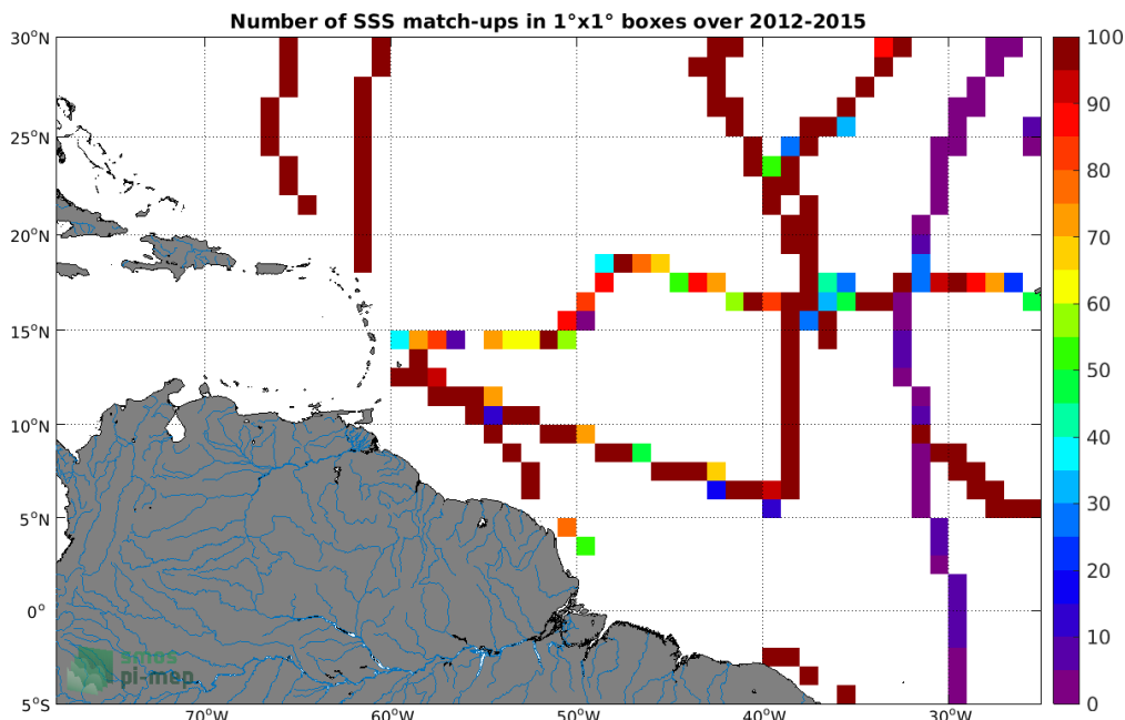
Figure 4: Number of SSS match-ups between TSG (GOSUD-Sailing-ship) SSS and the Aquarius SSS L3 CAP v5 - 7-Day running (JPL) SSS product for the Amazon and Orinoco river plumes Pi-MEP region over 1°x1° boxes and for the full satellite product period.
