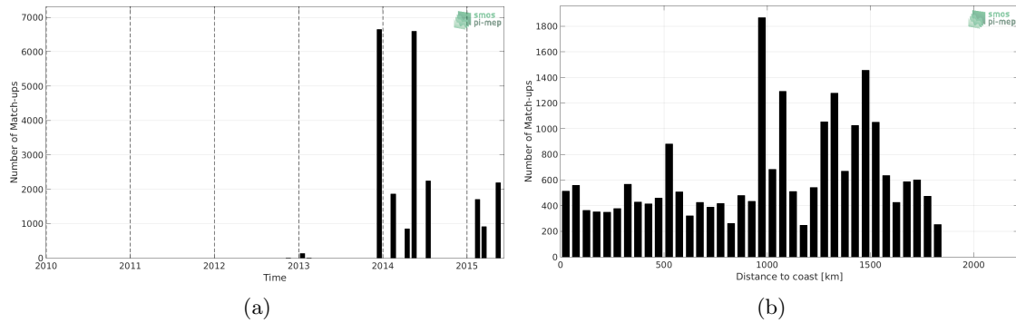
Figure 1: Number of match-ups between TSG-GOSUD-Sailing-ship and Aquarius-L3-JPL-V5-7DAY-RUNNING SSS as a function of time (a) and as function of the distance to coast (b) over the Amazon and Orinoco river plumes Pi-MEP region and for the full satellite product period.
