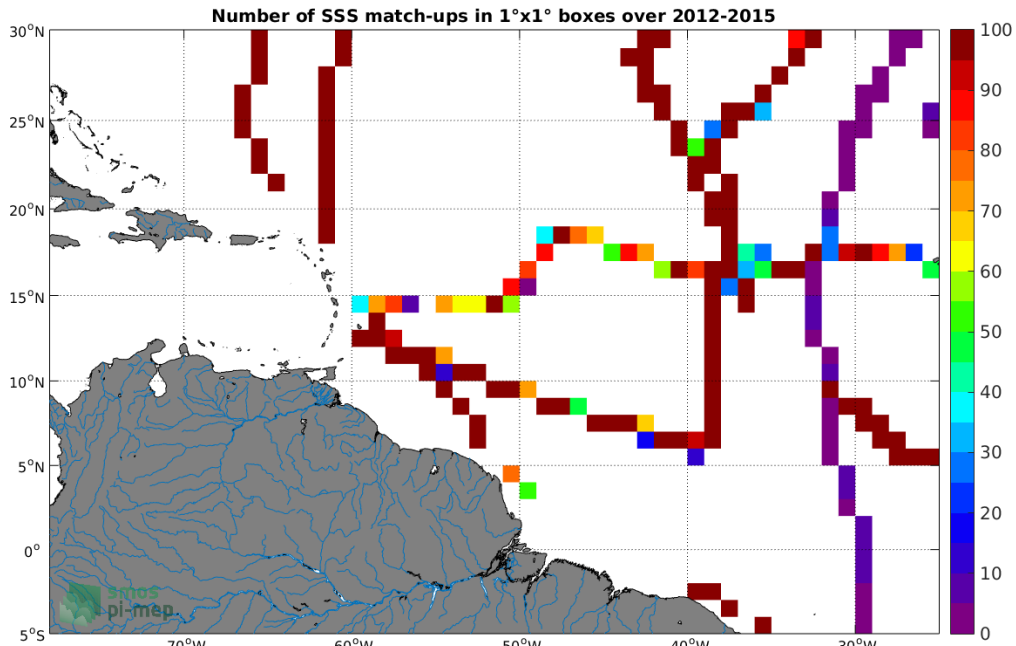
Figure 4: Number of SSS match-ups between TSG-GOSUD-Sailing-ship SSS and the Aquarius-L3-JPL-V5-7DAY-RUNNING SSS product for the Amazon and Orinoco river plumes Pi-MEP region over 1°x1° boxes and for the full satellite product period.
