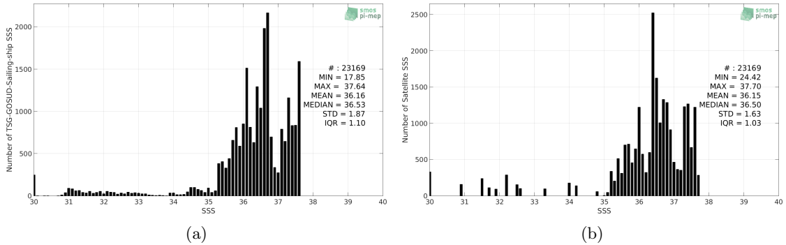
Figure 2: Histograms of SSS from TSG-GOSUD-Sailing-ship (a) and Aquarius-L3-JPL-V5-7DAY-RUNNING (b) considering all match-up pairs per bins of 0.1 over the Amazon and Orinoco river plumes Pi-MEP region and for the full satellite product period.
