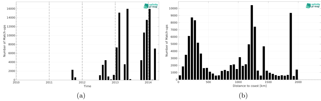
Figure 2: Number of match-ups between TSG (GOSUD-Research-vessel) and Aquarius SSS L3 CAP v5 - 7-Day running (JPL) SSS as a function of time (a) and as function of the distance to coast (b) over the Amazon and Orinoco river plumes Pi-MEP region and for the full satellite product period.
