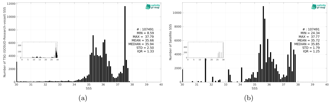
Figure 3: Histograms of SSS from TSG (GOSUD-Research-vessel) (a) and Aquarius SSS L3 CAP v5 - 7-Day running (JPL) (b) considering all match-up pairs per bins of 0.1 over the Amazon and Orinoco river plumes Pi-MEP region and for the full satellite product period.
