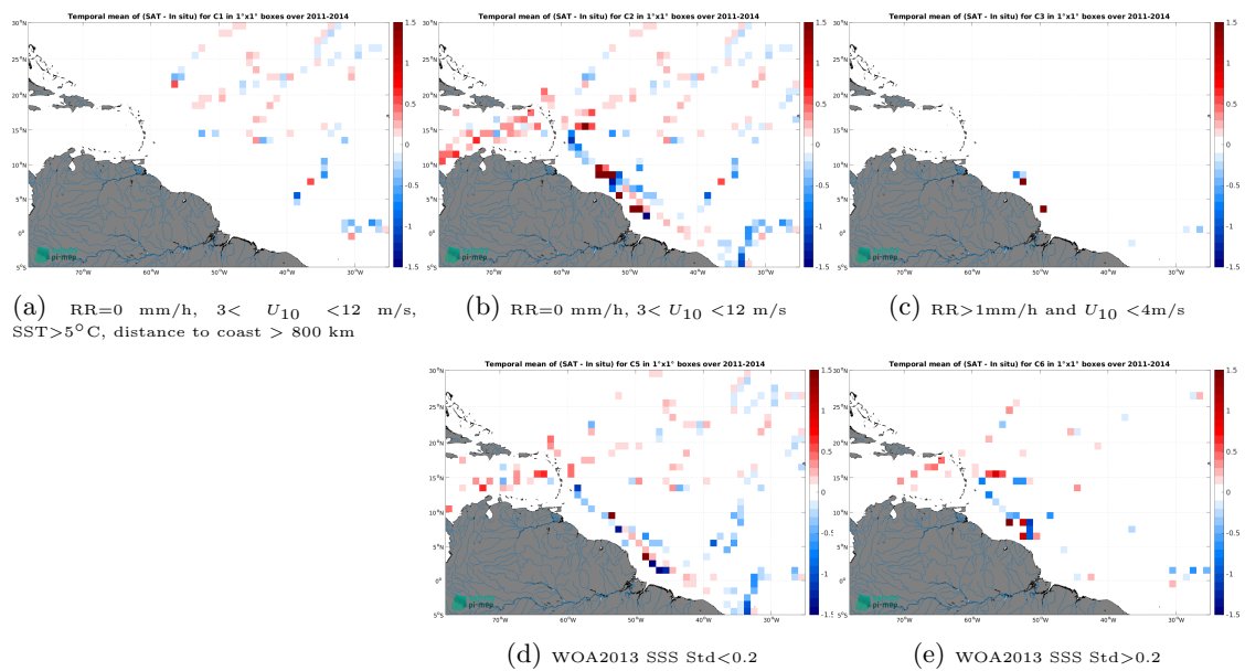
Figure 14: Temporal mean gridded over spatial boxes of size 1^\circ \times 1^\circ of \Delta SSS (Aquarius SSS L3 CAP v5 - 7-Day running (JPL) - TSG (GOSUD-Research-vessel)) for 5 different subdatasets corresponding to:RR=0 mm/h, 3 < U_{10} < 12 m/s, SST >5^\circ C, distance to coast > 800 km (a), RR=0 mm/h, 3 < U_{10} < 12 m/s (b), RR >1 mm/h and U_{10} < 4 m/s (c), WOA2013 SSS Std <0.2 (d), WOA2013 SSS Std >0.2 (e).
