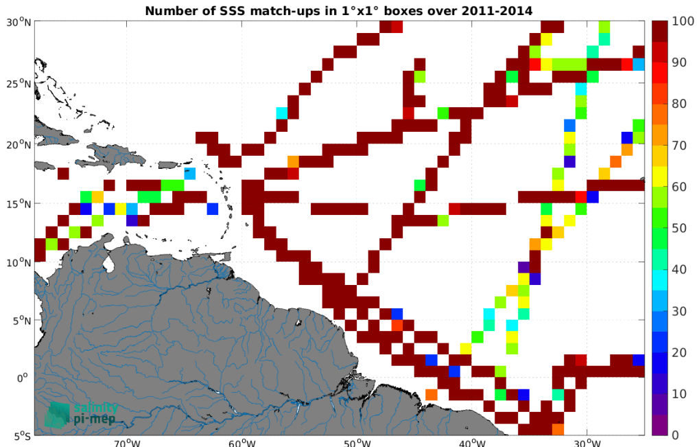
Figure 5: Number of SSS match-ups between TSG (GOSUD-Research-vessel) SSS and the Aquarius SSS L3 CAP v5 - 7-Day running (JPL) SSS product for the Amazon and Orinoco river plumes Pi-MEP region over 1^\circ \times 1^\circ boxes and for the full satellite product period.
