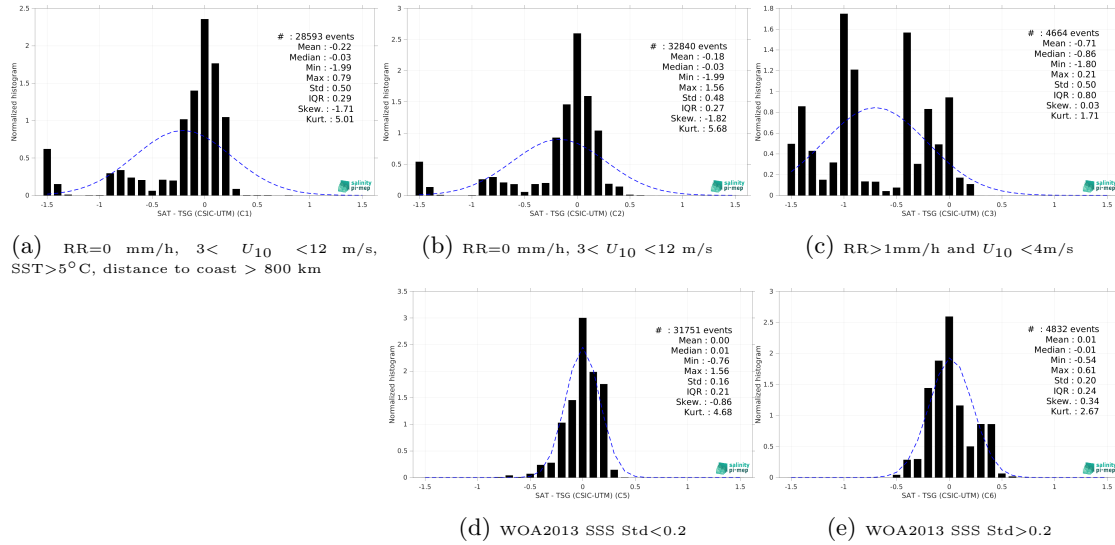
Figure 13: Normalized histogram of \Delta\text{SSS} (Aquarius SSS L3 CAP v5 - 7-Day running (JPL) - TSG (CSIC-UTM)) for 5 different subdatasets corresponding to: RR=0 mm/h, 3 < U_{10} < 12 m/s, SST>5°C, distance to coast > 800 km (a), RR=0 mm/h, 3 < U_{10} < 12 m/s (b), RR>1mm/h and U_{10} < 4 m/s (c), WOA2013 SSS Std<0.2 (d), WOA2013 SSS Std>0.2 (e).
