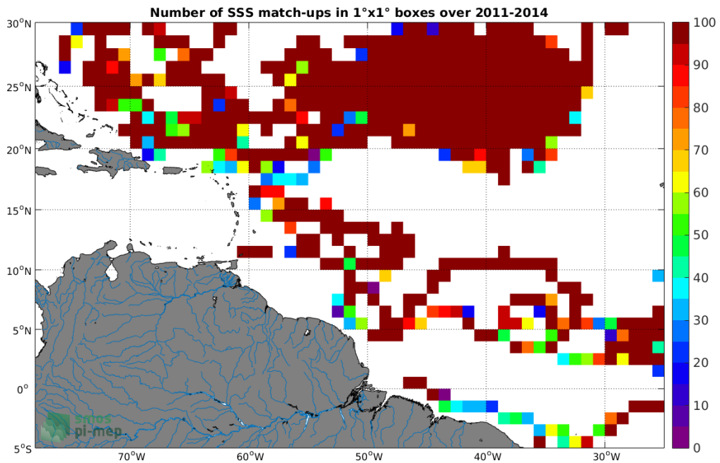
Figure 3: Number of SSS match-ups between Surface drifters SSS and the Aquarius-L3-JPL-V5-7DAY-RUNNING SSS product for the Amazon and Orinoco river plumes Pi-MEP region over 1°x1° boxes and for the full satellite product period.
