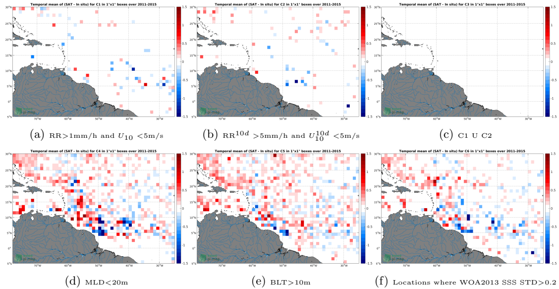
Figure 12: Temporal mean gridded over spatial boxes of size 1^\circ \times 1^\circ of \Delta SSS (Aquarius-L3-JPL-V5-7DAY-RUNNING - Argo) for 6 different subdatasets corresponding to: RR > 1\text{mm/h} and U_{10} < 5\text{m/s} (a), RR^{10d} > 5\text{mm/h} and U_{10}^{10d} < 5\text{m/s} (b), C1 U C2 (c), MLD < 20\text{m} (d), BLT > 10\text{m} (e), Locations where WOA2013 SSS STD > 0.2 (f).
