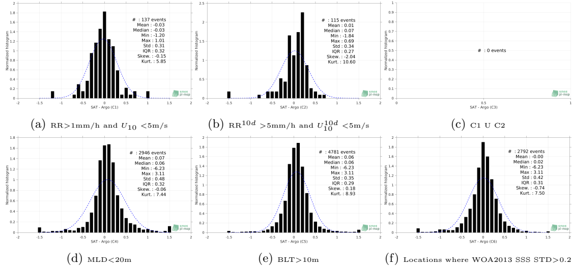
Figure 13: Normalized histogram of \Delta SSS (Aquarius-L3-JPL-V5-7DAY-RUNNING - Argo) for 6 different subdatasets corresponding to: RR>1mm/h and U_{10} < 5\text{m/s} (a), RR^{10d} > 5\text{mm/h} and U_{10}^{10d} < 5\text{m/s} (b), C1 U C2 (c), MLD<20m (d), BLT>10m (e), Locations where WOA2013 SSS STD>0.2 (f).
