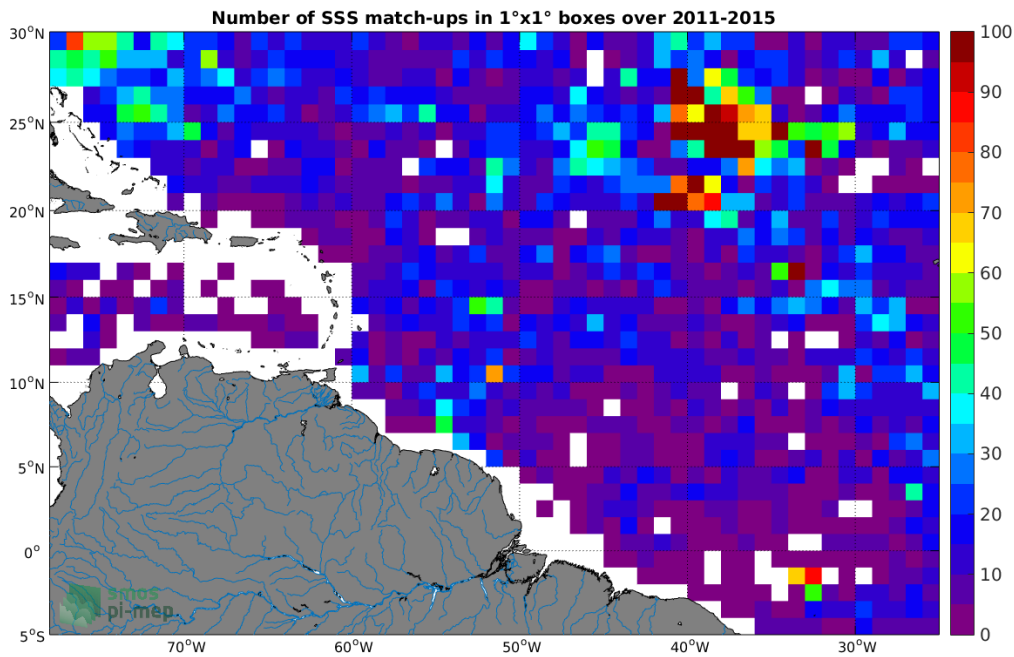
Figure 4: Number of SSS match-ups between Argo SSS and the Aquarius-L3-JPL-V5-7DAY-RUNNING SSS product for the Amazon and Orinoco river plumes Pi-MEP region over 1^{\circ} \times 1^{\circ} boxes and for the full satellite product period.
