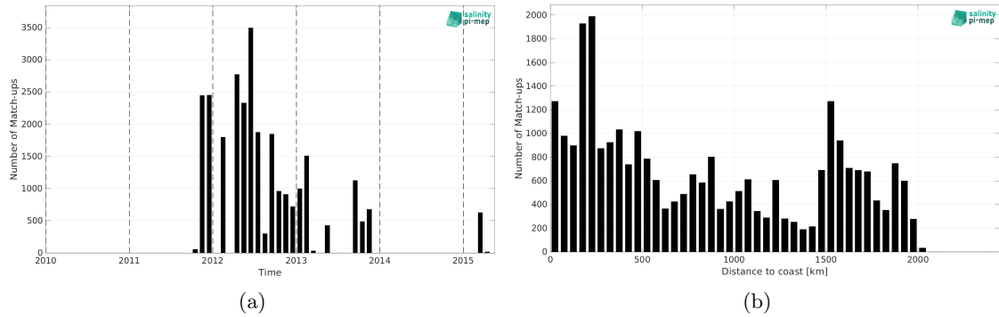
Figure 2: Number of match-ups between TSG (SAMOS) and Aquarius SSS L3 CAP v5 - Monthly (JPL) SSS as a function of time (a) and as function of the distance to coast (b) over the Amazon and Orinoco river plumes Pi-MEP region and for the full satellite product period.
