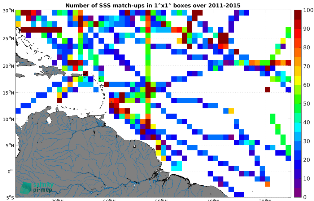
Figure 5: Number of SSS match-ups between TSG (SAMOS) SSS and the Aquarius SSS L3 CAP v5 - Monthly (JPL) SSS product for the Amazon and Orinoco river plumes Pi-MEP region over 1^\circ \times 1^\circ boxes and for the full satellite product period.
