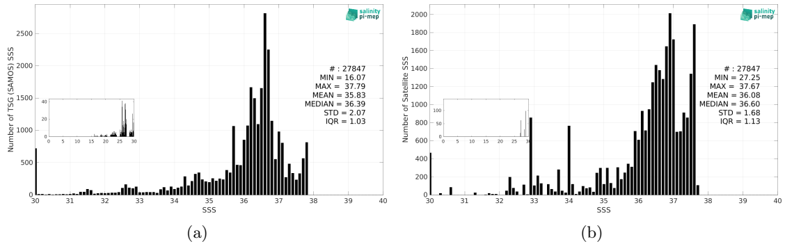
Figure 3: Histograms of SSS from TSG (SAMOS) (a) and Aquarius SSS L3 CAP v5 - Monthly (JPL) (b) considering all match-up pairs per bins of 0.1 over the Amazon and Orinoco river plumes Pi-MEP region and for the full satellite product period.
