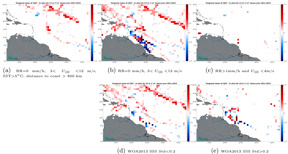
Figure 12: Temporal mean gridded over spatial boxes of size 1^\circ \times 1^\circ of \Delta\text{SSS} (Aquarius SSS L3 CAP v5 - Monthly (JPL) - TSG (SAMOS)) for 5 different subdatasets corresponding to:RR=0 mm/h, 3 < U_{10} < 12 m/s, SST >5^\circ\text{C} , distance to coast > 800 km (a), RR=0 mm/h, 3 < U_{10} < 12 m/s (b), RR >1 mm/h and U_{10} < 4 m/s (c), WOA2013 SSS Std <0.2 (d), WOA2013 SSS Std >0.2 (e).
