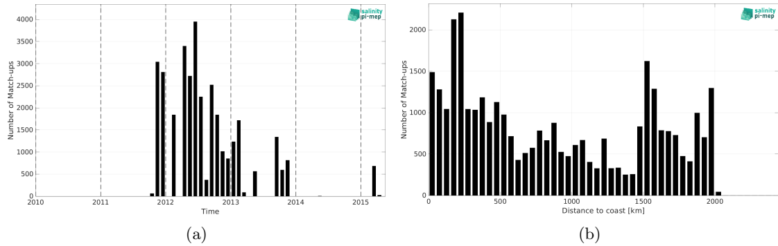
Figure 1: Number of match-ups between TSG (SAMOS) and Aquarius SSS L3 CAP v5 - Monthly (JPL) SSS as a function of time (a) and as function of the distance to coast (b) over the Amazon and Orinoco river plumes Pi-MEP region and for the full satellite product period.
