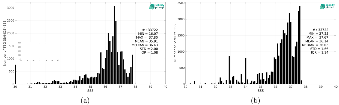
Figure 2: Histograms of SSS from TSG (SAMOS) (a) and Aquarius SSS L3 CAP v5 - Monthly (JPL) (b) considering all match-up pairs per bins of 0.1 over the Amazon and Orinoco river plumes Pi-MEP region and for the full satellite product period.
