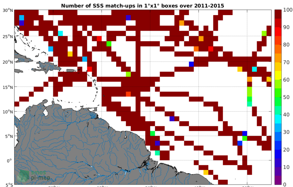
Figure 4: Number of SSS match-ups between TSG-SAMOS SSS and the Aquarius-L3-JPL-V5-MONTHLY SSS product for the Amazon and Orinoco river plumes Pi-MEP region over 1^{\circ} \times 1^{\circ} boxes and for the full satellite product period.
