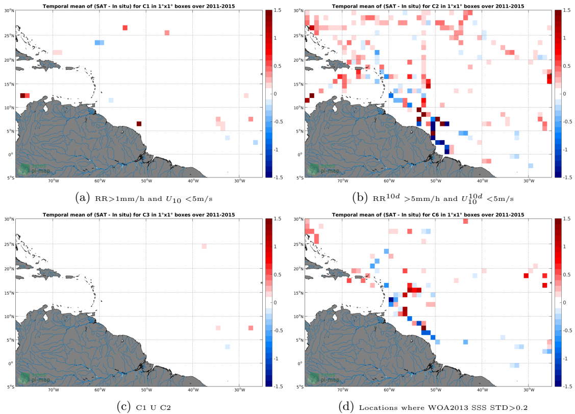
Figure 12: Temporal mean gridded over spatial boxes of size 1^\circ \times 1^\circ of \Delta SSS (Aquarius-L3-JPL-V5-MONTHLY - TSG-SAMOS) for 4 different subdatasets corresponding to: RR > 1 mm/h and U_{10} < 5 m/s (a), RR 10d > 5 mm/h and U_{10}^{10d} < 5 m/s (b), C1 U C2 (c), Locations where WOA2013 SSS STD > 0.2 (d).
