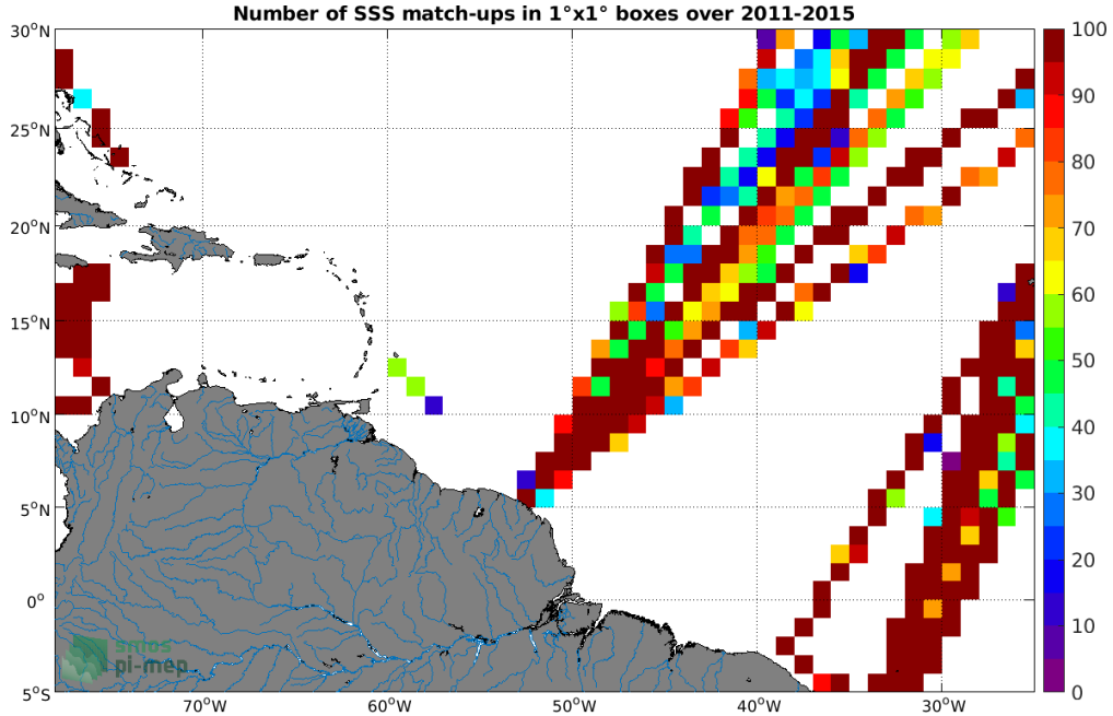
Figure 4: Number of SSS match-ups between TSG (LEGOS-DM) SSS and the Aquarius SSS L3 CAP v5 - Monthly (JPL) SSS product for the Amazon and Orinoco river plumes Pi-MEP region over 1^\circ \times 1^\circ boxes and for the full satellite product period.
