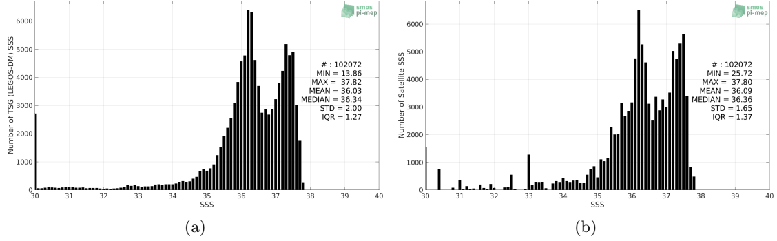
Figure 2: Histograms of SSS from TSG (LEGOS-DM) (a) and Aquarius SSS L3 CAP v5 - Monthly (JPL) (b) considering all match-up pairs per bins of 0.1 over the Amazon and Orinoco river plumes Pi-MEP region and for the full satellite product period.
