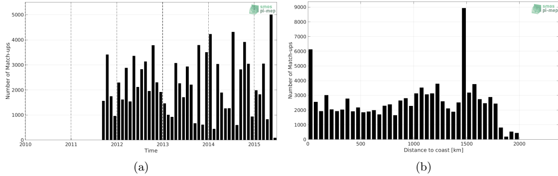
Figure 1: Number of match-ups between TSG (LEGOS-DM) and Aquarius SSS L3 CAP v5 - Monthly (JPL) SSS as a function of time (a) and as function of the distance to coast (b) over the Amazon and Orinoco river plumes Pi-MEP region and for the full satellite product period.
