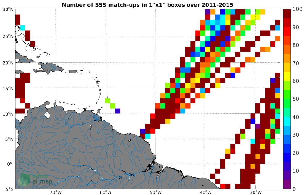
Figure 4: Number of SSS match-ups between TSG (LEGOS-DM) SSS and the Aquarius SSS L3 CAP v5 - Monthly (JPL) SSS product for the Amazon and Orinoco river plumes Pi-MEP region over 1°x1° boxes and for the full satellite product period.
