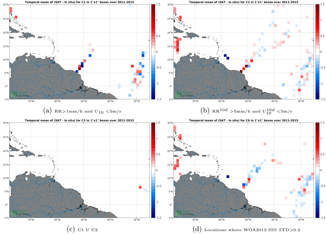
Figure 12: Temporal mean gridded over spatial boxes of size 1^\circ \times 1^\circ of \Delta SSS (Aquarius-L3-JPL-V5-MONTHLY - TSG-LEGOS-DM) for 4 different subdatasets corresponding to: RR > 1mm/h and U_{10} < 5\text{m/s} (a), RR^{10d} > 5\text{mm/h} and U_{10}^{10d} < 5\text{m/s} (b), C1 U C2 (c), Locations where WOA2013 SSS STD > 0.2 (d).
