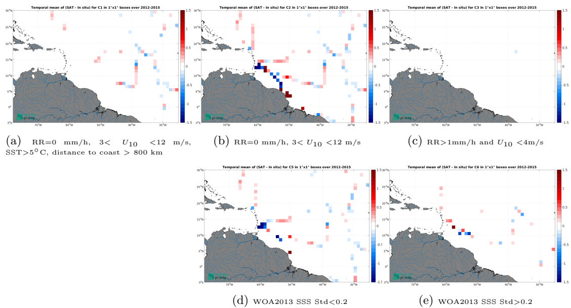
Figure 14: Temporal mean gridded over spatial boxes of size 1^\circ \times 1^\circ of \Delta SSS (Aquarius SSS L3 CAP v5 - Monthly (JPL) - TSG (GOSUD-Sailing-ship)) for 5 different subdatasets corresponding to:RR=0 mm/h, 3 < U_{10} < 12 m/s, SST >5^\circ\text{C} , distance to coast > 800 km (a), RR=0 mm/h, 3 < U_{10} < 12 m/s (b), RR >1 mm/h and U_{10} < 4 m/s (c), WOA2013 SSS Std <0.2 (d), WOA2013 SSS Std >0.2 (e).
