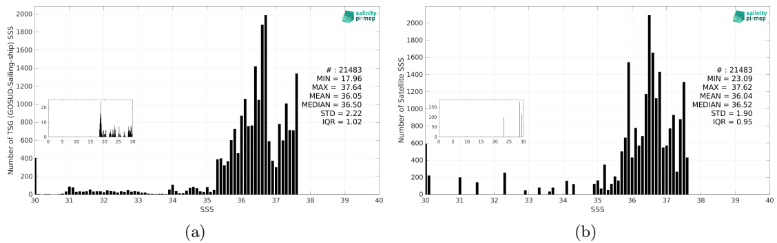
Figure 3: Histograms of SSS from TSG (GOSUD-Sailing-ship) (a) and Aquarius SSS L3 CAP v5 - Monthly (JPL) (b) considering all match-up pairs per bins of 0.1 over the Amazon and Orinoco river plumes Pi-MEP region and for the full satellite product period.
