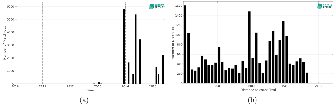
Figure 2: Number of match-ups between TSG (GOSUD-Sailing-ship) and Aquarius SSS L3 CAP v5 - Monthly (JPL) SSS as a function of time (a) and as function of the distance to coast (b) over the Amazon and Orinoco river plumes Pi-MEP region and for the full satellite product period.
