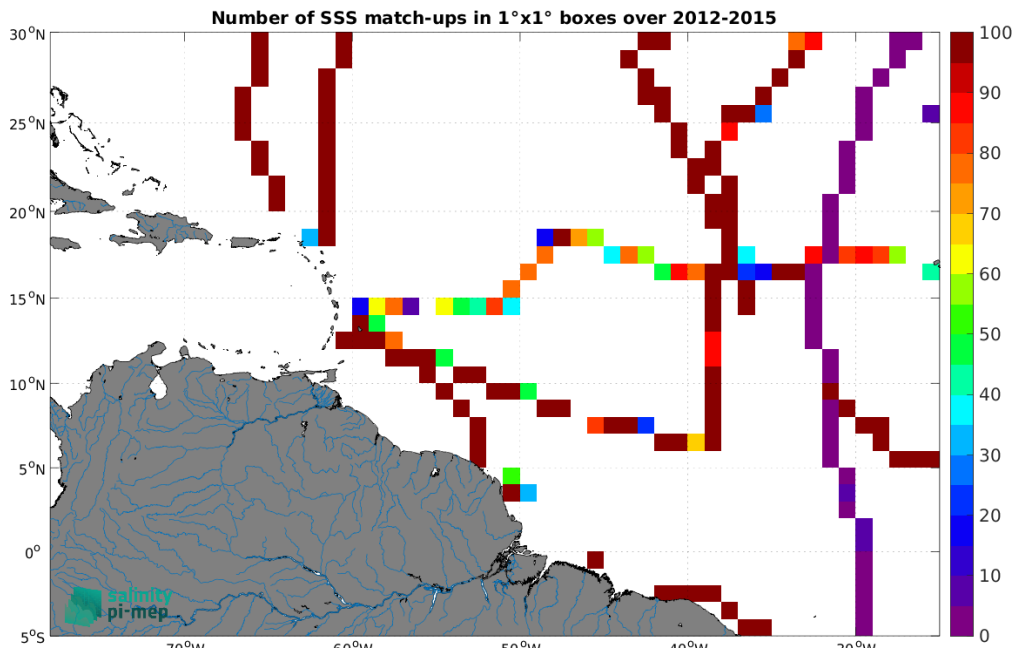
Figure 5: Number of SSS match-ups between TSG (GOSUD-Sailing-ship) SSS and the Aquarius SSS L3 CAP v5 - Monthly (JPL) SSS product for the Amazon and Orinoco river plumes Pi-MEP region over 1^\circ \times 1^\circ boxes and for the full satellite product period.
