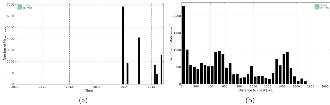
Figure 1: Number of match-ups between TSG-GOSUD-Sailing-ship and Aquarius-L3-JPL-V5-MONTHLY SSS as a function of time (a) and as function of the distance to coast (b) over the Amazon and Orinoco river plumes Pi-MEP region and for the full satellite product period.
