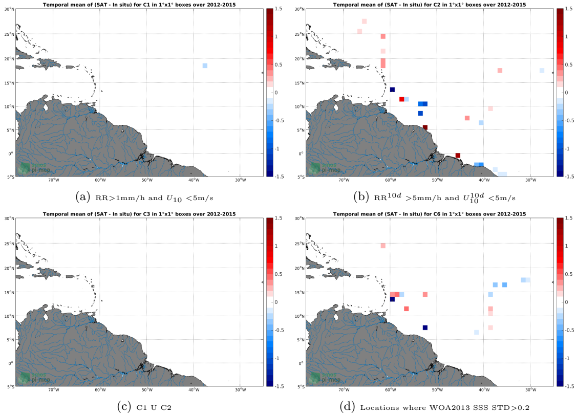
Figure 12: Temporal mean gridded over spatial boxes of size 1^\circ \times 1^\circ of \Delta SSS (Aquarius-L3-JPL-V5-MONTHLY - TSG-GOSUD-Sailing-ship) for 4 different subdatasets corresponding to: RR > 1\text{mm/h} and U_{10} < 5\text{m/s} (a), RR^{10d} > 5\text{mm/h} and U_{10}^{10d} < 5\text{m/s} (b), C1 U C2 (c), Locations where WOA2013 SSS STD > 0.2 (d).
