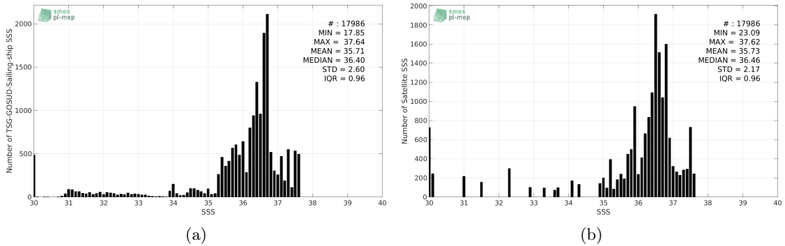
Figure 2: Histograms of SSS from TSG-GOSUD-Sailing-ship (a) and Aquarius-L3-JPL-V5-MONTHLY (b) considering all match-up pairs per bins of 0.1 over the Amazon and Orinoco river plumes Pi-MEP region and for the full satellite product period.
