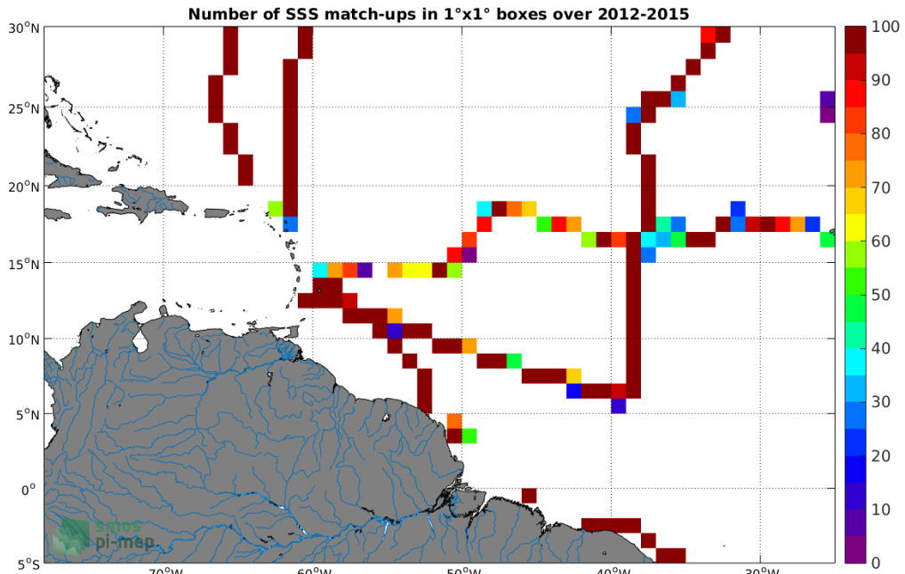
Figure 4: Number of SSS match-ups between TSG-GOSUD-Sailing-ship SSS and the Aquarius-L3-JPL-V5-MONTHLY SSS product for the Amazon and Orinoco river plumes Pi-MEP region over 1°x1° boxes and for the full satellite product period.
