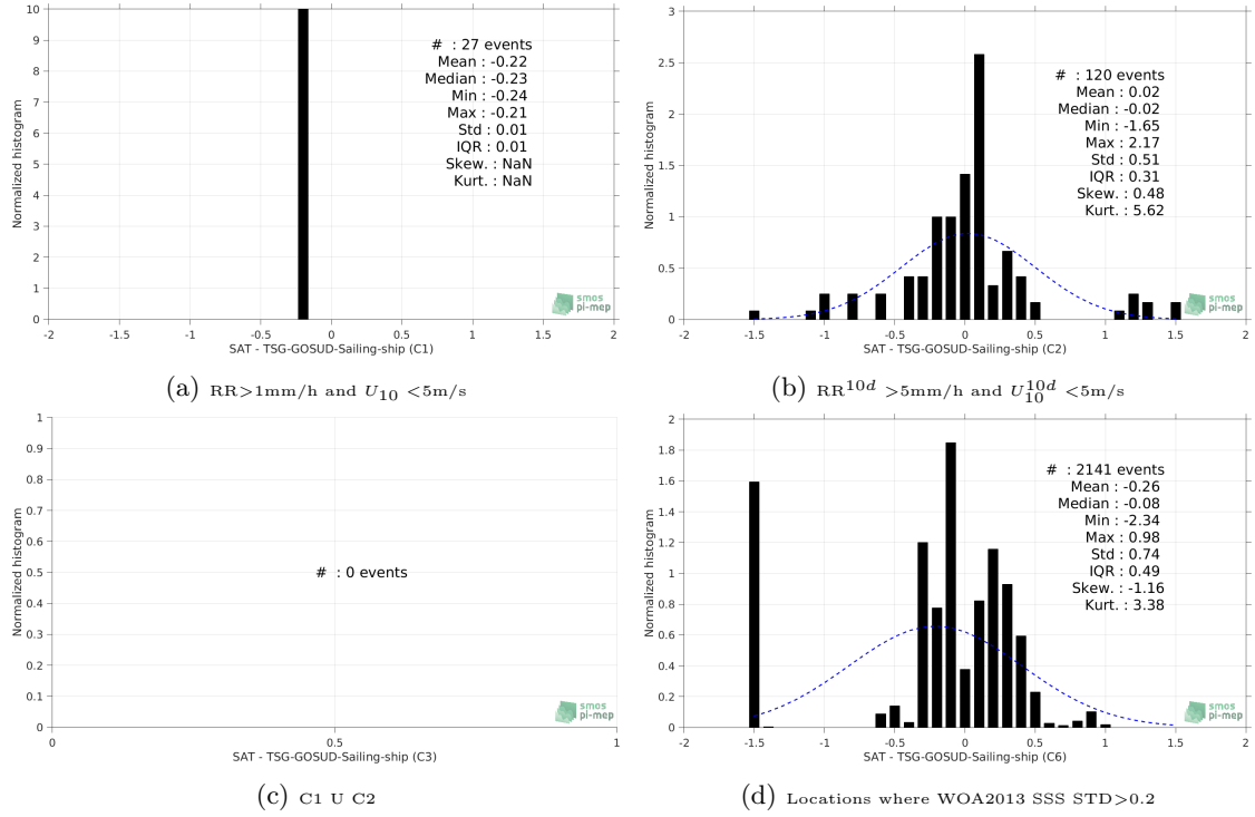
Figure 13: Normalized histogram of \Delta\text{SSS} (Aquarius-L3-JPL-V5-MONTHLY - TSG-GOSUD-Sailing-ship) for 6 different subdatasets corresponding to: RR > 1\text{mm/h} and U_{10} < 5\text{m/s} (a), RR^{10d} > 5\text{mm/h} and U_{10}^{10d} < 5\text{m/s} (b), C1 U C2 (c), Locations where WOA2013 SSS STD > 0.2 (d).
