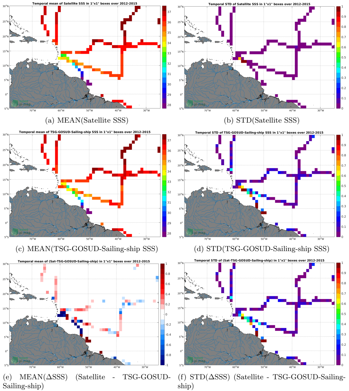
Figure 6: Temporal mean (left) and STD (right) of SSS from Aquarius-L3-JPL-V5-MONTHLY (top), TSG-GOSUD-Sailing-ship (middle), and of \Delta SSS (Satellite - TSG-GOSUD-Sailing-ship). Only match-up pairs are used to generate these maps.
