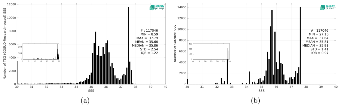
Figure 3: Histograms of SSS from TSG (GOSUD-Research-vessel) (a) and Aquarius SSS L3 CAP v5 - Monthly (JPL) (b) considering all match-up pairs per bins of 0.1 over the Amazon and Orinoco river plumes Pi-MEP region and for the full satellite product period.
