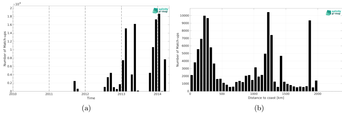
Figure 2: Number of match-ups between TSG (GOSUD-Research-vessel) and Aquarius SSS L3 CAP v5 - Monthly (JPL) SSS as a function of time (a) and as function of the distance to coast (b) over the Amazon and Orinoco river plumes Pi-MEP region and for the full satellite product period.
