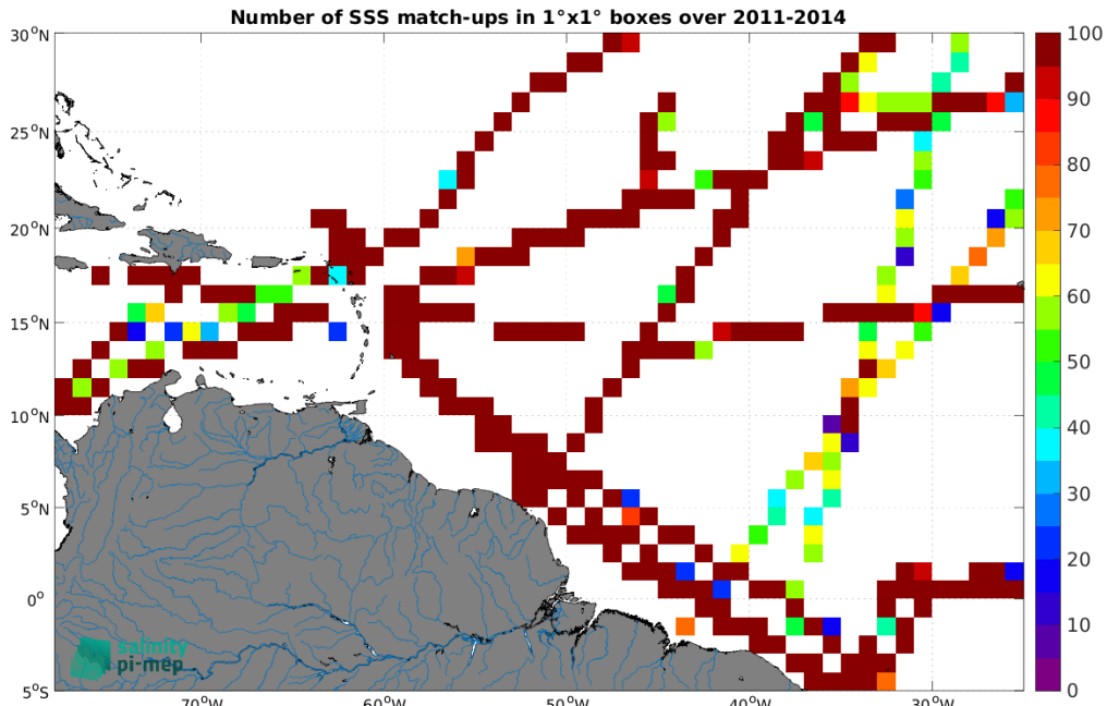
Figure 5: Number of SSS match-ups between TSG (GOSUD-Research-vessel) SSS and the Aquarius SSS L3 CAP v5 - Monthly (JPL) SSS product for the Amazon and Orinoco river plumes Pi-MEP region over 1^\circ \times 1^\circ boxes and for the full satellite product period.
