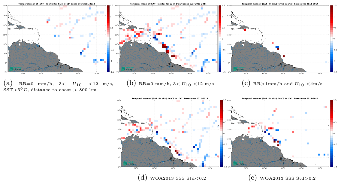
Figure 14: Temporal mean gridded over spatial boxes of size 1^\circ \times 1^\circ of \Delta SSS (Aquarius SSS L3 CAP v5 - Monthly (JPL) - TSG (GOSUD-Research-vessel)) for 5 different subdatasets corresponding to:RR=0 mm/h, 3 < U_{10} < 12 m/s, SST>5°C, distance to coast > 800 km (a), RR=0 mm/h, 3 < U_{10} < 12 m/s (b), RR>1mm/h and U_{10} < 4 m/s (c), WOA2013 SSS Std<0.2 (d), WOA2013 SSS Std>0.2 (e).
