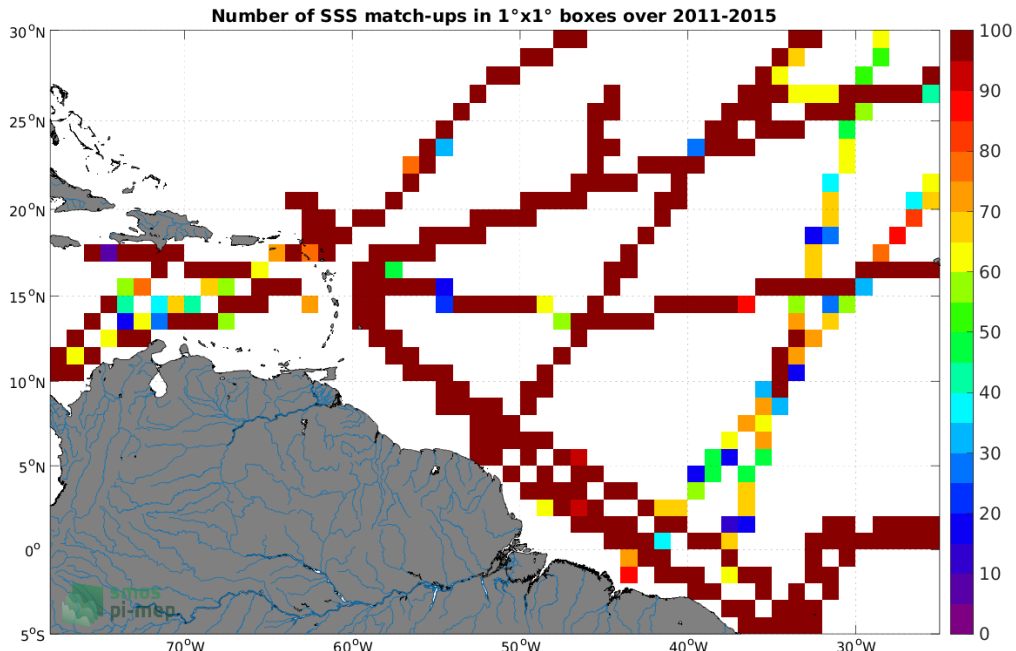
Figure 4: Number of SSS match-ups between TSG (GOSUD-Research-vessel) SSS and the Aquarius SSS L3 CAP v5 - Monthly (JPL) SSS product for the Amazon and Orinoco river plumes Pi-MEP region over 1°×1° boxes and for the full satellite product period.
