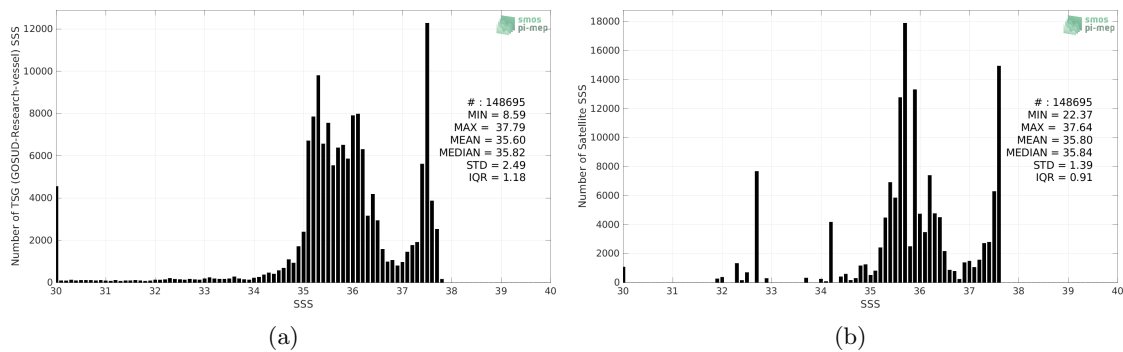
Figure 2: Histograms of SSS from TSG (GOSUD-Research-vessel) (a) and Aquarius SSS L3 CAP v5 - Monthly (JPL) (b) considering all match-up pairs per bins of 0.1 over the Amazon and Orinoco river plumes Pi-MEP region and for the full satellite product period.
