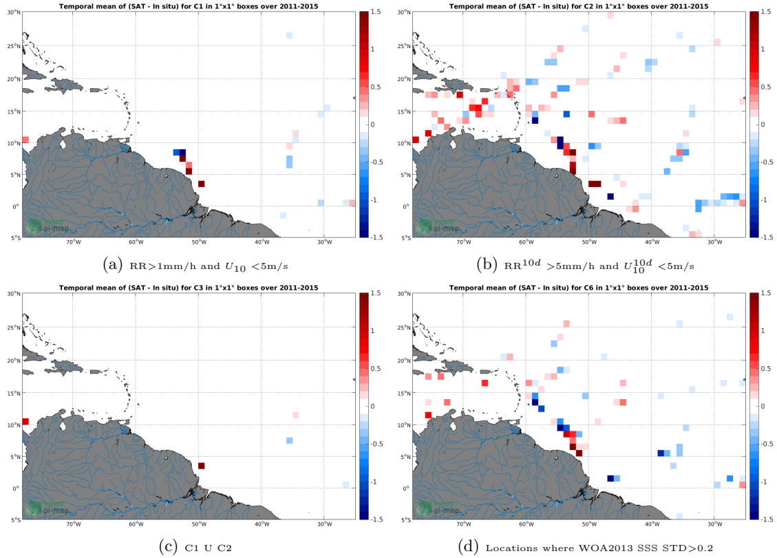
Figure 12: Temporal mean gridded over spatial boxes of size 1^\circ \times 1^\circ of \Delta SSS (Aquarius-L3-JPL-V5-MONTHLY - TSG-GOSUD-Research-vessel) for 4 different subdatasets corresponding to: RR > 1\text{mm/h} and U_{10} < 5\text{m/s} (a), RR^{10d} > 5\text{mm/h} and U_{10}^{10d} < 5\text{m/s} (b), C1 U C2 (c), Locations where WOA2013 SSS STD > 0.2 (d).
