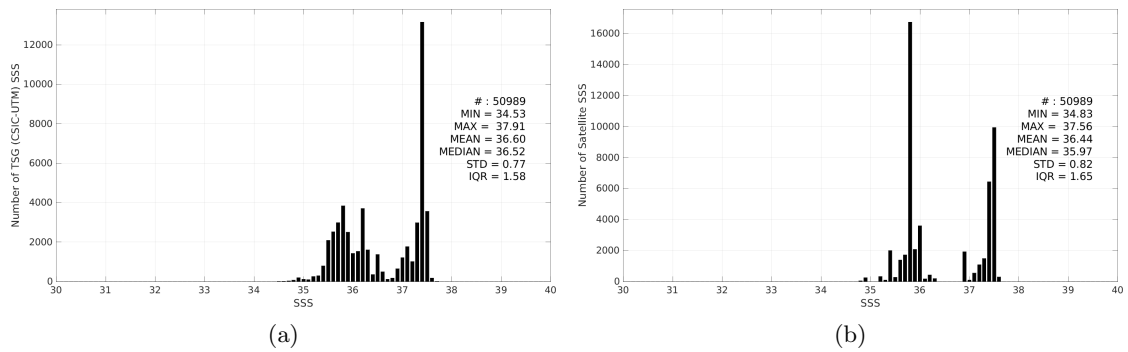
Figure 3: Histograms of SSS from TSG (CSIC-UTM) (a) and Aquarius SSS L3 CAP v5 - Monthly (JPL) (b) considering all match-up pairs per bins of 0.1 over the Amazon and Orinoco river plumes Pi-MEP region and for the full satellite product period.
