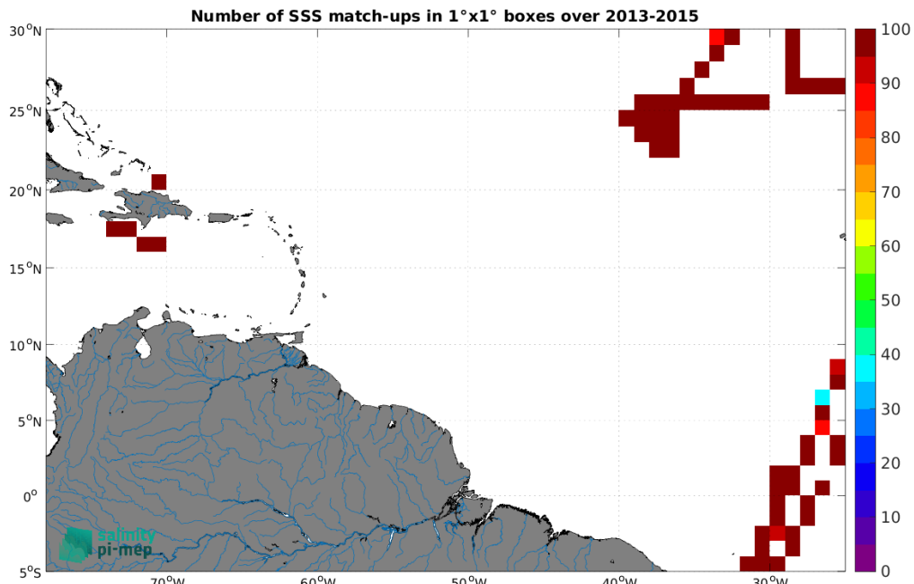
Figure 5: Number of SSS match-ups between TSG (CSIC-UTM) SSS and the Aquarius SSS L3 CAP v5 - Monthly (JPL) SSS product for the Amazon and Orinoco river plumes Pi-MEP region over 1^\circ \times 1^\circ boxes and for the full satellite product period.
