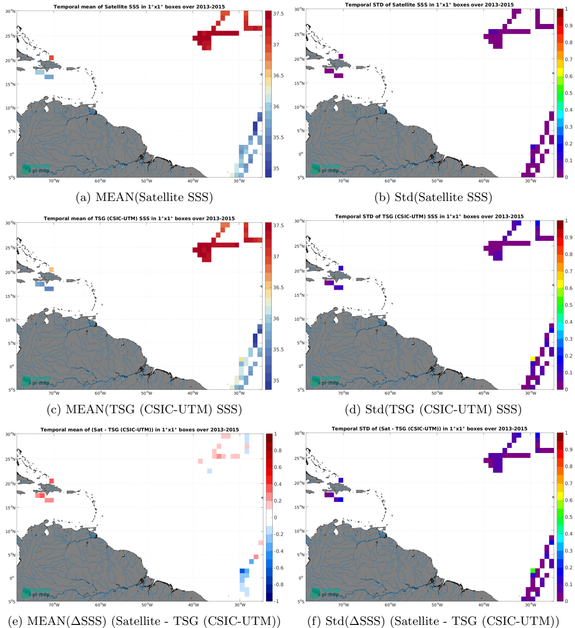
Figure 7: Temporal mean (left) and Std (right) of SSS from Aquarius SSS L3 CAP v5 - Monthly (JPL) (top), TSG (CSIC-UTM) (middle), and of \Delta SSS (Satellite - TSG (CSIC-UTM)). Only match-up pairs are used to generate these maps.
