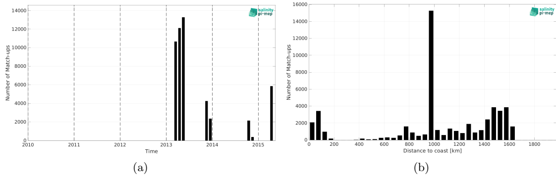
Figure 2: Number of match-ups between TSG (CSIC-UTM) and Aquarius SSS L3 CAP v5 - Monthly (JPL) SSS as a function of time (a) and as function of the distance to coast (b) over the Amazon and Orinoco river plumes Pi-MEP region and for the full satellite product period.
