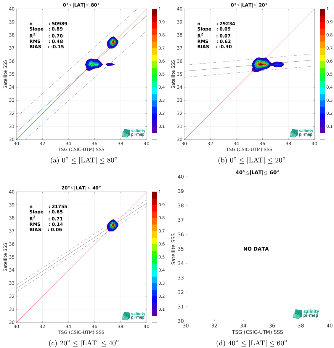
Figure 10: Contour maps of the concentration of Aquarius SSS L3 CAP v5 - Monthly (JPL) SSS (y-axis) versus TSG (CSIC-UTM) SSS (x-axis) at match-up pairs for different latitude bands. For each plot, the red line shows x=y . The black thin and dashed lines indicate a linear fit through the data cloud and the \pm 95\% confidence levels, respectively. The number match-up pairs n , the slope and R^2 coefficient of the linear fit, the root mean square (RMS) and the mean bias between satellite and in situ data are indicated for each latitude band in each plots.
