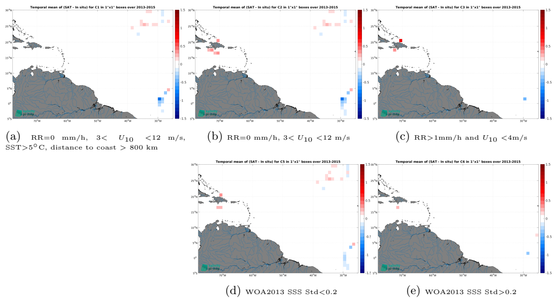
Figure 14: Temporal mean gridded over spatial boxes of size 1^\circ \times 1^\circ of \Delta SSS (Aquarius SSS L3 CAP v5 - Monthly (JPL) - TSG (CSIC-UTM)) for 5 different subdatasets corresponding to:RR=0 mm/h, 3 < U_{10} < 12 m/s, SST >5^\circ C, distance to coast > 800 km (a), RR=0 mm/h, 3 < U_{10} < 12 m/s (b), RR >1 mm/h and U_{10} < 4 m/s (c), WOA2013 SSS Std <0.2 (d), WOA2013 SSS Std >0.2 (e).
