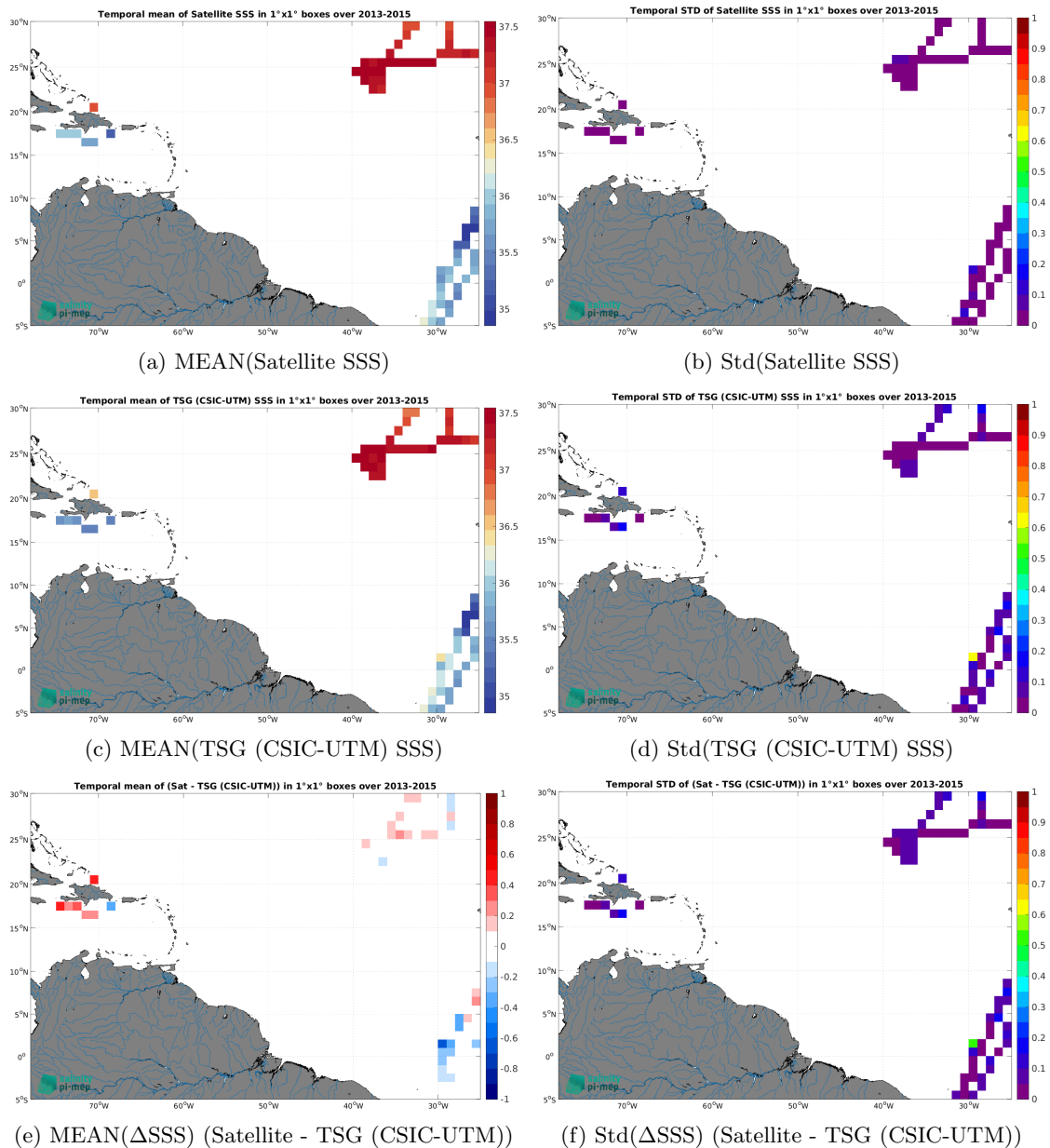
Figure 6: Temporal mean (left) and Std (right) of SSS from Aquarius SSS L3 CAP v5 - Monthly (JPL) (top), TSG (CSIC-UTM) (middle), and of \Delta SSS (Satellite - TSG (CSIC-UTM)). Only match-up pairs are used to generate these maps.
