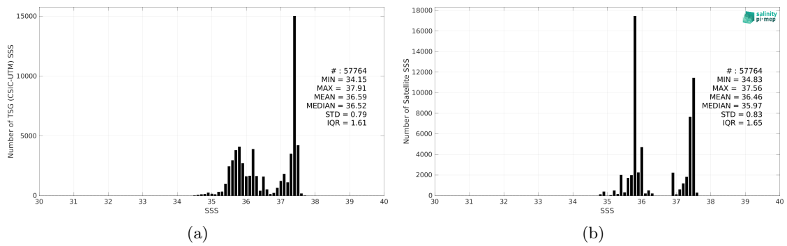
Figure 2: Histograms of SSS from TSG (CSIC-UTM) (a) and Aquarius SSS L3 CAP v5 - Monthly (JPL) (b) considering all match-up pairs per bins of 0.1 over the Amazon and Orinoco river plumes Pi-MEP region and for the full satellite product period.
