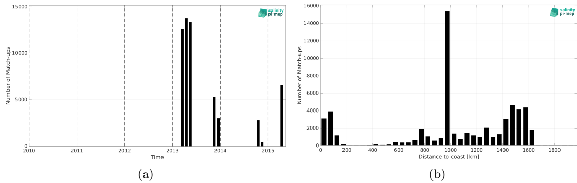
Figure 1: Number of match-ups between TSG (CSIC-UTM) and Aquarius SSS L3 CAP v5 - Monthly (JPL) SSS as a function of time (a) and as function of the distance to coast (b) over the Amazon and Orinoco river plumes Pi-MEP region and for the full satellite product period.
