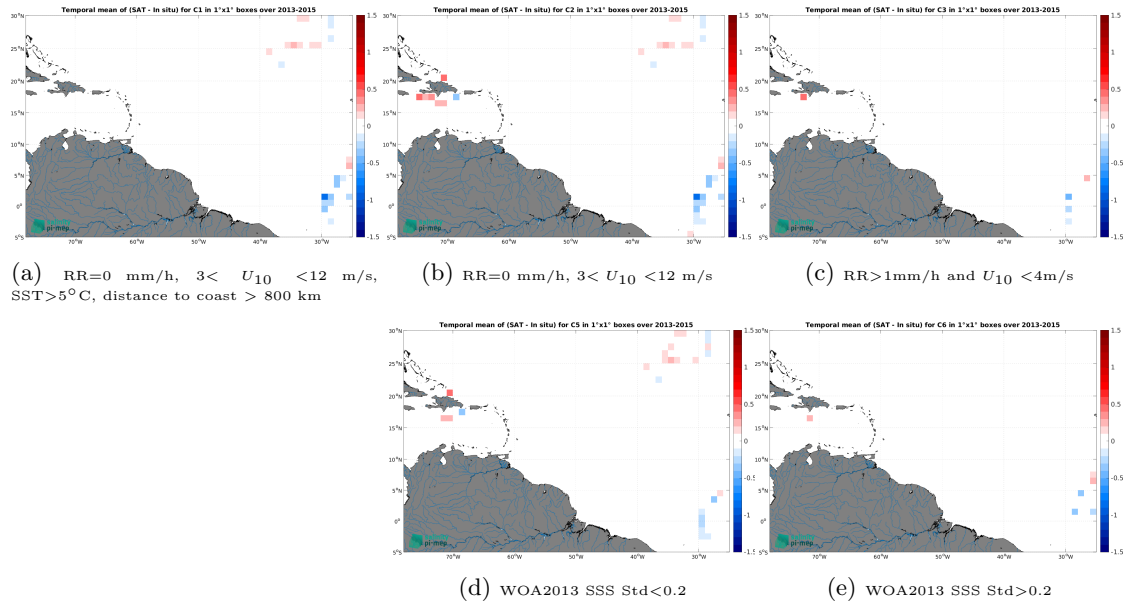
Figure 12: Temporal mean gridded over spatial boxes of size 1^\circ \times 1^\circ of \Delta SSS (Aquarius SSS L3 CAP v5 - Monthly (JPL) - TSG (CSIC-UTM)) for 5 different subdatasets corresponding to:RR=0 mm/h, 3 < U_{10} < 12 m/s, SST >5^\circ C, distance to coast > 800 km (a), RR=0 mm/h, 3 < U_{10} < 12 m/s (b), RR >1 mm/h and U_{10} < 4 m/s (c), WOA2013 SSS Std <0.2 (d), WOA2013 SSS Std >0.2 (e).
