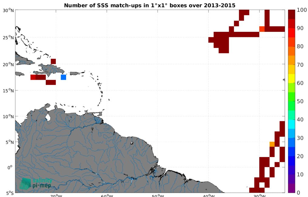
Figure 4: Number of SSS match-ups between TSG (CSIC-UTM) SSS and the Aquarius SSS L3 CAP v5 - Monthly (JPL) SSS product for the Amazon and Orinoco river plumes Pi-MEP region over 1^\circ \times 1^\circ boxes and for the full satellite product period.
