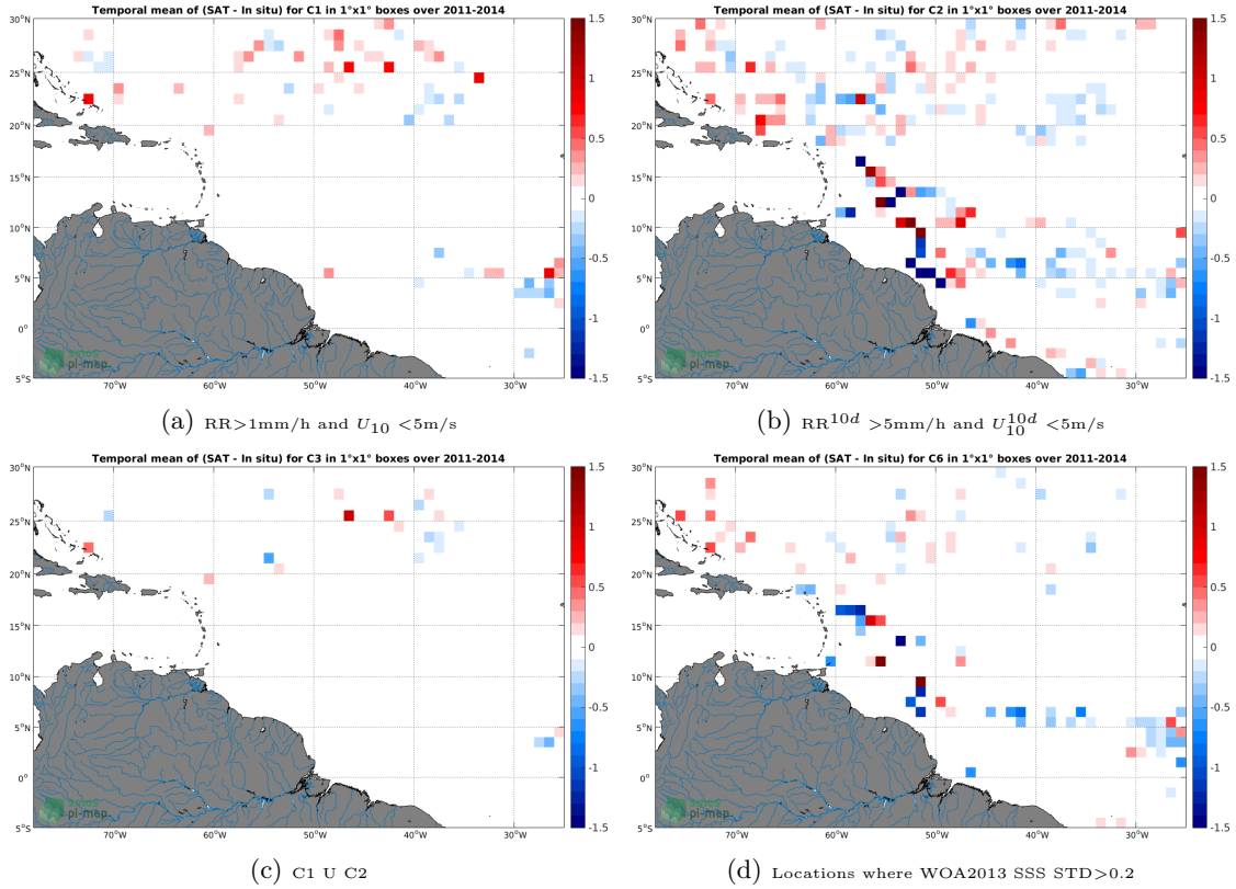
Figure 11: Temporal mean gridded over spatial boxes of size 1^\circ \times 1^\circ of \Delta SSS (Aquarius-L3-JPL-V5-MONTHLY - Surface drifters) for 4 different subdatasets corresponding to: RR > 1\text{mm/h} and U_{10} < 5\text{m/s} (a), RR^{10d} > 5\text{mm/h} and U_{10}^{10d} < 5\text{m/s} (b), C1 U C2 (c), Locations where WOA2013 SSS STD > 0.2 (d).
