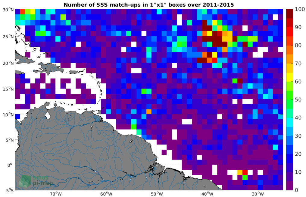
Figure 4: Number of SSS match-ups between Argo SSS and the Aquarius SSS L3 CAP v5 - Monthly (JPL) SSS product for the Amazon and Orinoco river plumes Pi-MEP region over 1^{\circ} \times 1^{\circ} boxes and for the full satellite product period.
