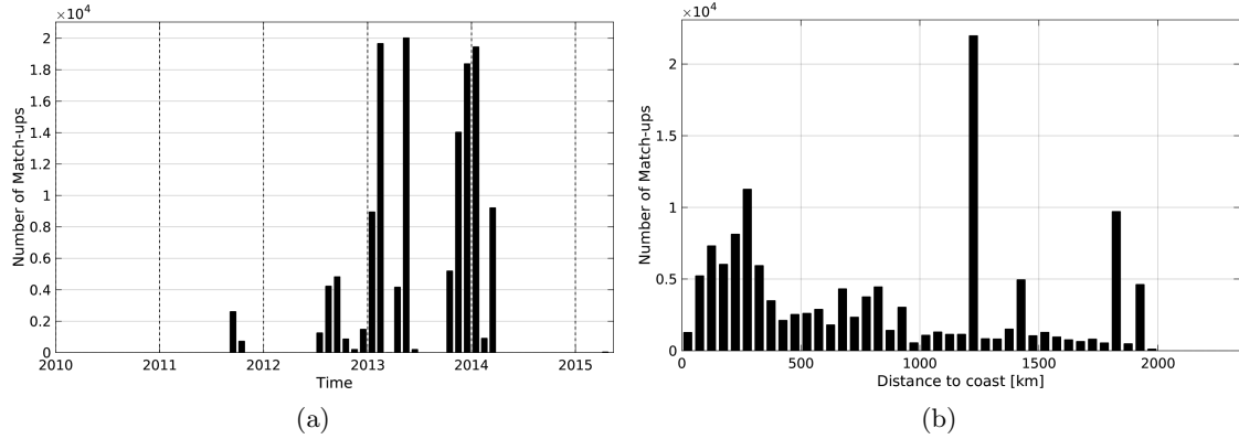
Figure 1: Number of match-ups between TSG-GOSUD-Research-vessel and Aquarius-L3-JPL-V4-7DAY-RUNNING SSS as a function of time (a) and as function of the distance to coast (b) over the Amazon and Orinoco river plumes Pi-MEP region and for the full satellite product period.
