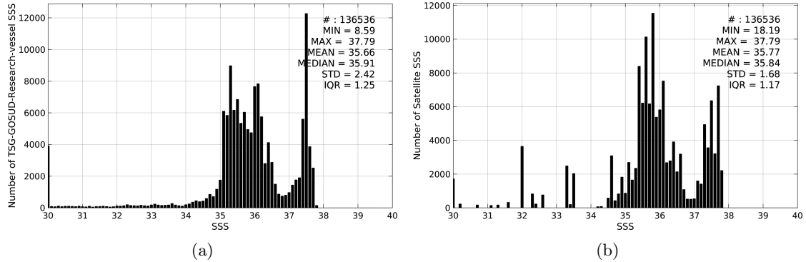
Figure 2: Histograms of SSS from TSG-GOSUD-Research-vessel (a) and Aquarius-L3-JPL-V4-7DAY-RUNNING (b) considering all match-up pairs per bins of 0.1 over the Amazon and Orinoco river plumes Pi-MEP region and for the full satellite product period.
