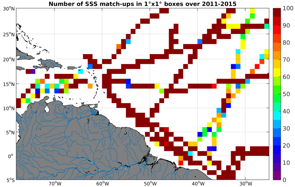
Figure 4: Number of SSS match-ups between TSG-GOSUD-Research-vessel SSS and the Aquarius-L3-JPL-V4-7DAY-RUNNING SSS product for the Amazon and Orinoco river plumes Pi-MEP region over 1^\circ \times 1^\circ boxes and for the full satellite product period.
