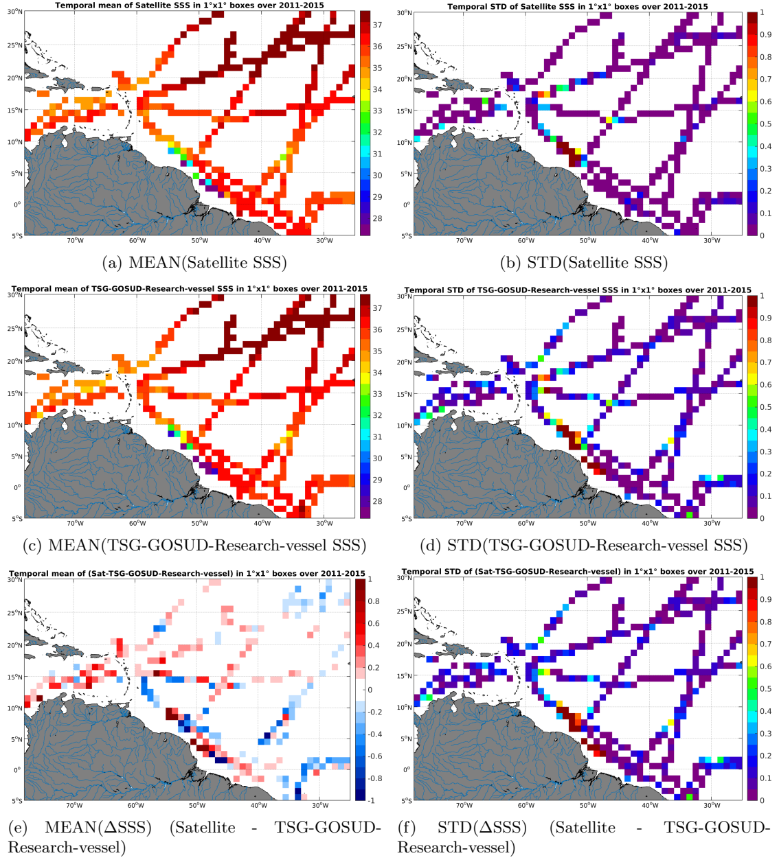
Figure 6: Temporal mean (left) and STD (right) of SSS from Aquarius-L3-JPL-V4-7DAY-RUNNING (top), TSG-GOSUD-Research-vessel (middle), and of \Delta SSS (Satellite - TSG-GOSUD-Research-vessel). Only match-up pairs are used to generate these maps.
