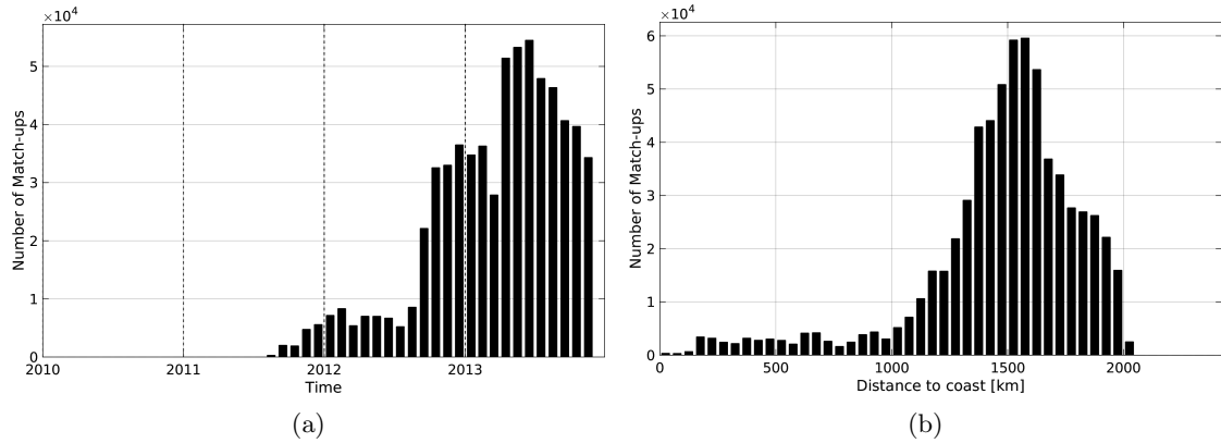
Figure 1: Number of match-ups between Surface drifters and Aquarius-L3-JPL-V4-7DAY-RUNNING SSS as a function of time (a) and as function of the distance to coast (b) over the Amazon and Orinoco river plumes Pi-MEP region and for the full satellite product period.
