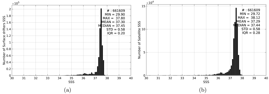
Figure 2: Histograms of SSS from Surface drifters (a) and Aquarius-L3-JPL-V4-7DAY-RUNNING (b) considering all match-up pairs per bins of 0.1 over the Amazon and Orinoco river plumes Pi-MEP region and for the full satellite product period.
