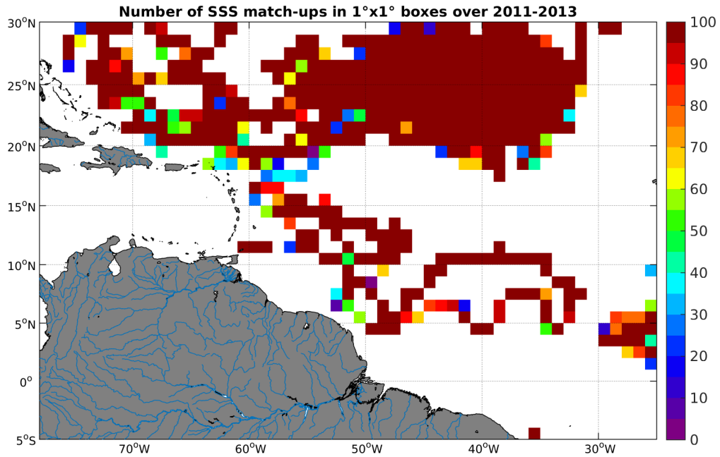
Figure 3: Number of SSS match-ups between Surface drifters SSS and the Aquarius-L3-JPL-V4-7DAY-RUNNING SSS product for the Amazon and Orinoco river plumes Pi-MEP region over 1°x1° boxes and for the full satellite product period.
