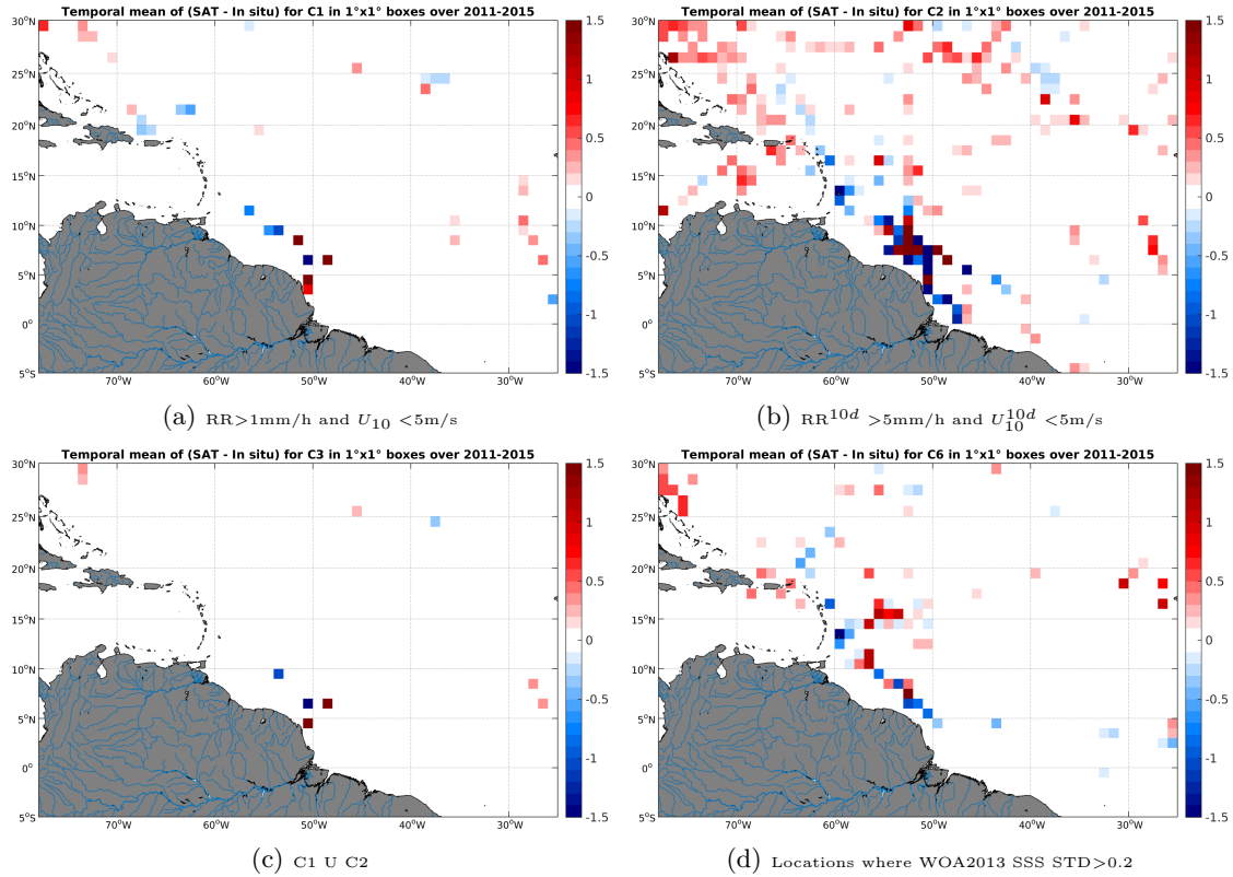
Figure 12: Temporal mean gridded over spatial boxes of size 1^\circ \times 1^\circ of \Delta SSS (Aquarius-L3-JPL-V4-MONTHLY - TSG-SAMOS) for 4 different subdatasets corresponding to: RR > 1 mm/h and U_{10} < 5 m/s (a), RR 10d > 5 mm/h and U_{10}^{10d} < 5 m/s (b), C1 U C2 (c), Locations where WOA2013 SSS STD > 0.2 (d).
