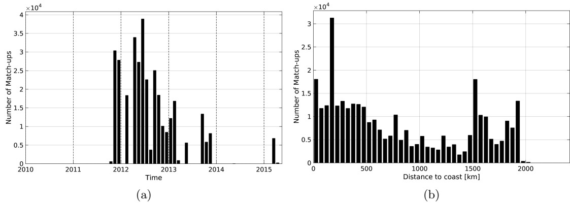
Figure 1: Number of match-ups between TSG-SAMOS and Aquarius-L3-JPL-V4-MONTHLY SSS as a function of time (a) and as function of the distance to coast (b) over the Amazon and Orinoco river plumes Pi-MEP region and for the full satellite product period.
