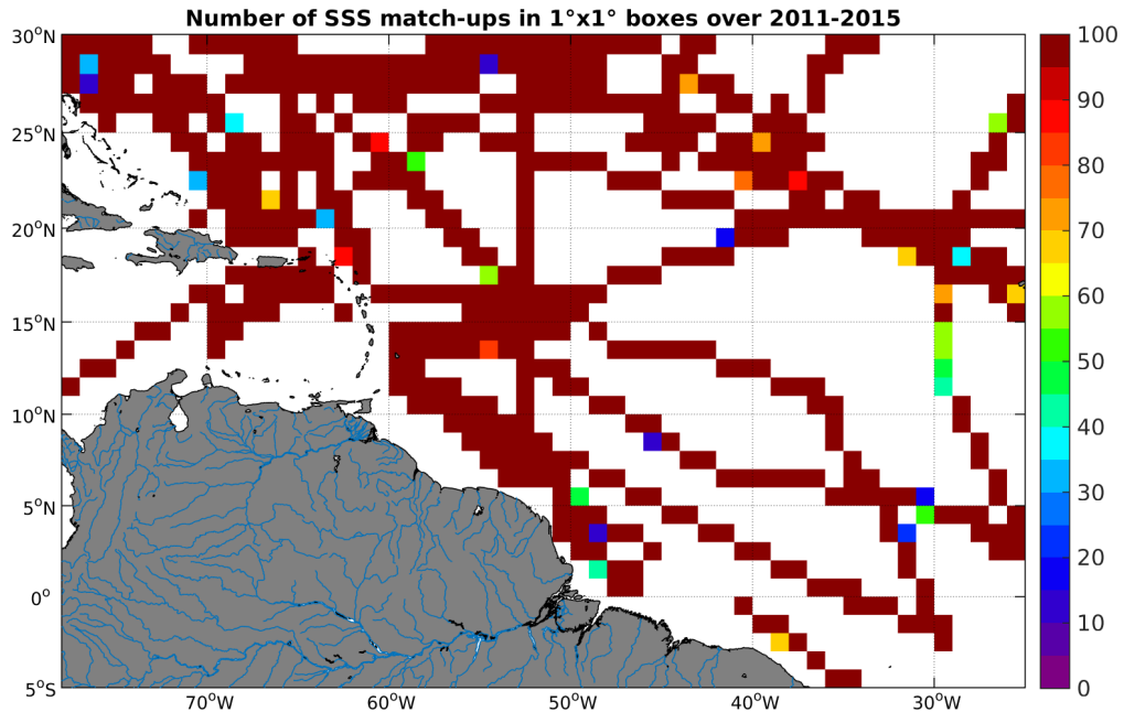
Figure 4: Number of SSS match-ups between TSG-SAMOS SSS and the Aquarius-L3-JPL-V4-MONTHLY SSS product for the Amazon and Orinoco river plumes Pi-MEP region over 1^\circ \times 1^\circ boxes and for the full satellite product period.
