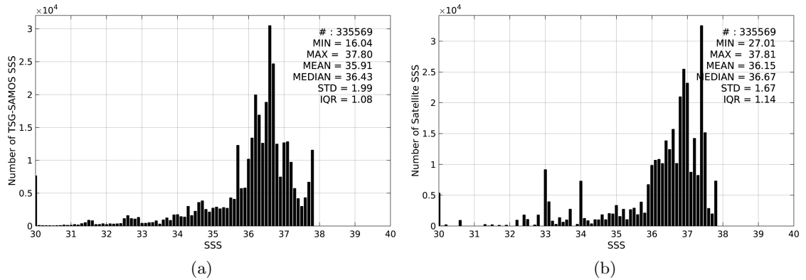
Figure 2: Histograms of SSS from TSG-SAMOS (a) and Aquarius-L3-JPL-V4-MONTHLY (b) considering all match-up pairs per bins of 0.1 over the Amazon and Orinoco river plumes Pi-MEP region and for the full satellite product period.
