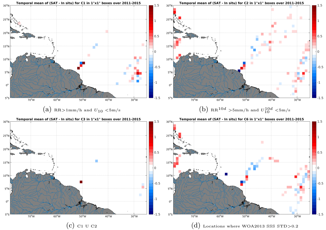
Figure 12: Temporal mean gridded over spatial boxes of size 1^\circ \times 1^\circ of \Delta SSS (Aquarius-L3-JPL-V4-MONTHLY - TSG-LEGOS-DM) for 4 different subdatasets corresponding to: RR > 1 mm/h and U_{10} < 5 m/s (a), RR^{10d} > 5 mm/h and U_{10}^{10d} < 5 m/s (b), C1 U C2 (c), Locations where WOA2013 SSS STD > 0.2 (d).
