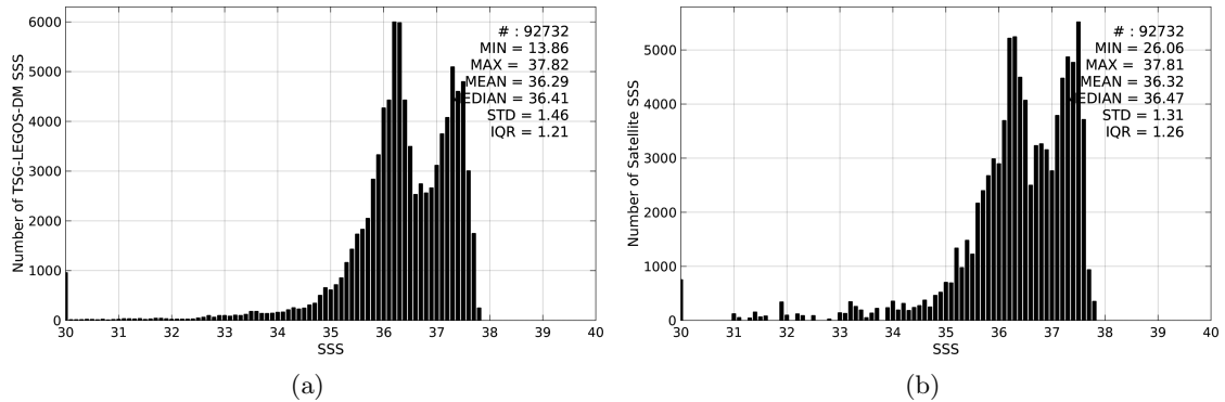
Figure 2: Histograms of SSS from TSG-LEGOS-DM (a) and Aquarius-L3-JPL-V4-MONTHLY (b) considering all match-up pairs per bins of 0.1 over the Amazon and Orinoco river plumes Pi-MEP region and for the full satellite product period.
