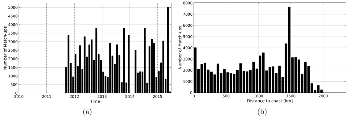
Figure 1: Number of match-ups between TSG-LEGOS-DM and Aquarius-L3-JPL-V4-MONTHLY SSS as a function of time (a) and as function of the distance to coast (b) over the Amazon and Orinoco river plumes Pi-MEP region and for the full satellite product period.
