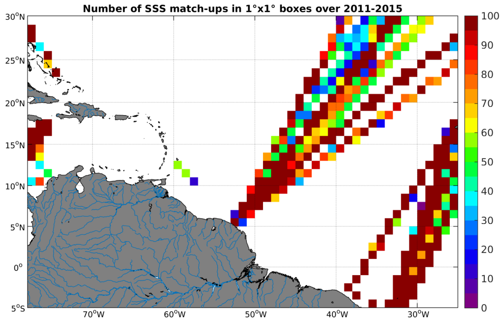
Figure 4: Number of SSS match-ups between TSG-LEGOS-DM SSS and the Aquarius-L3-JPL-V4-MONTHLY SSS product for the Amazon and Orinoco river plumes Pi-MEP region over 1^\circ \times 1^\circ boxes and for the full satellite product period.
