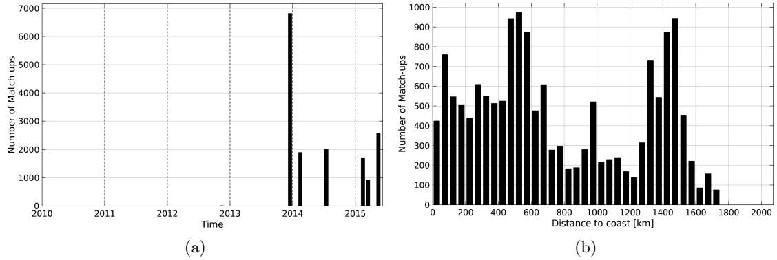
Figure 1: Number of match-ups between TSG-GOSUD-Sailing-ship and Aquarius-L3-JPL-V4-MONTHLY SSS as a function of time (a) and as function of the distance to coast (b) over the Amazon and Orinoco river plumes Pi-MEP region and for the full satellite product period.
