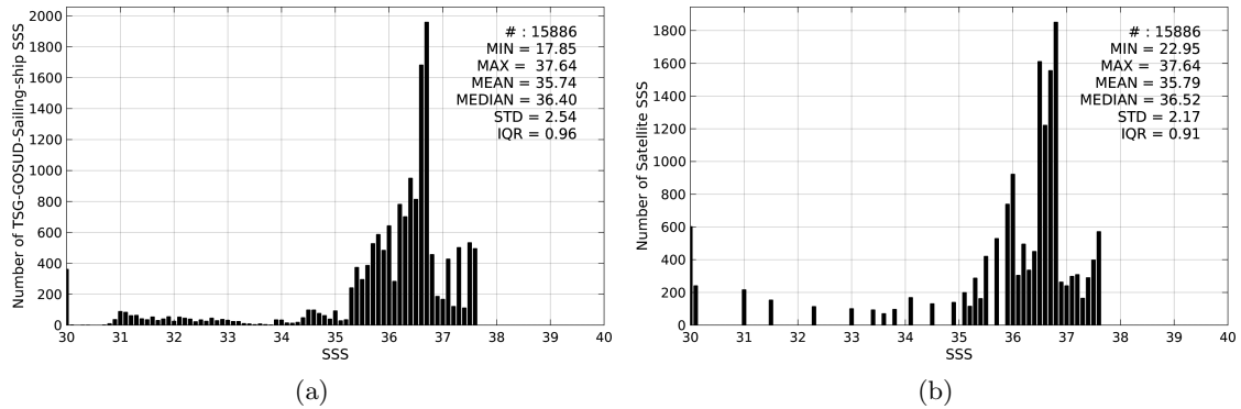
Figure 2: Histograms of SSS from TSG-GOSUD-Sailing-ship (a) and Aquarius-L3-JPL-V4-MONTHLY (b) considering all match-up pairs per bins of 0.1 over the Amazon and Orinoco river plumes Pi-MEP region and for the full satellite product period.
