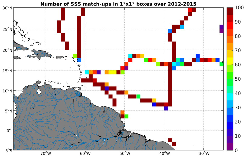
Figure 4: Number of SSS match-ups between TSG-GOSUD-Sailing-ship SSS and the Aquarius-L3-JPL-V4-MONTHLY SSS product for the Amazon and Orinoco river plumes Pi-MEP region over 1^\circ \times 1^\circ boxes and for the full satellite product period.
