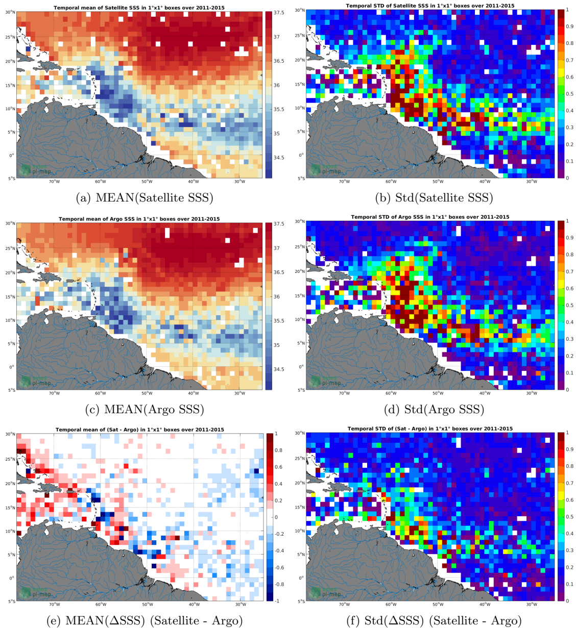
Figure 6: Temporal mean (left) and Std (right) of SSS from Aquarius SSS L2-AVERAGED OR v5 (NASA-GSFC) (top), Argo (middle), and of \Delta SSS (Satellite - Argo). Only match-up pairs are used to generate these maps.
