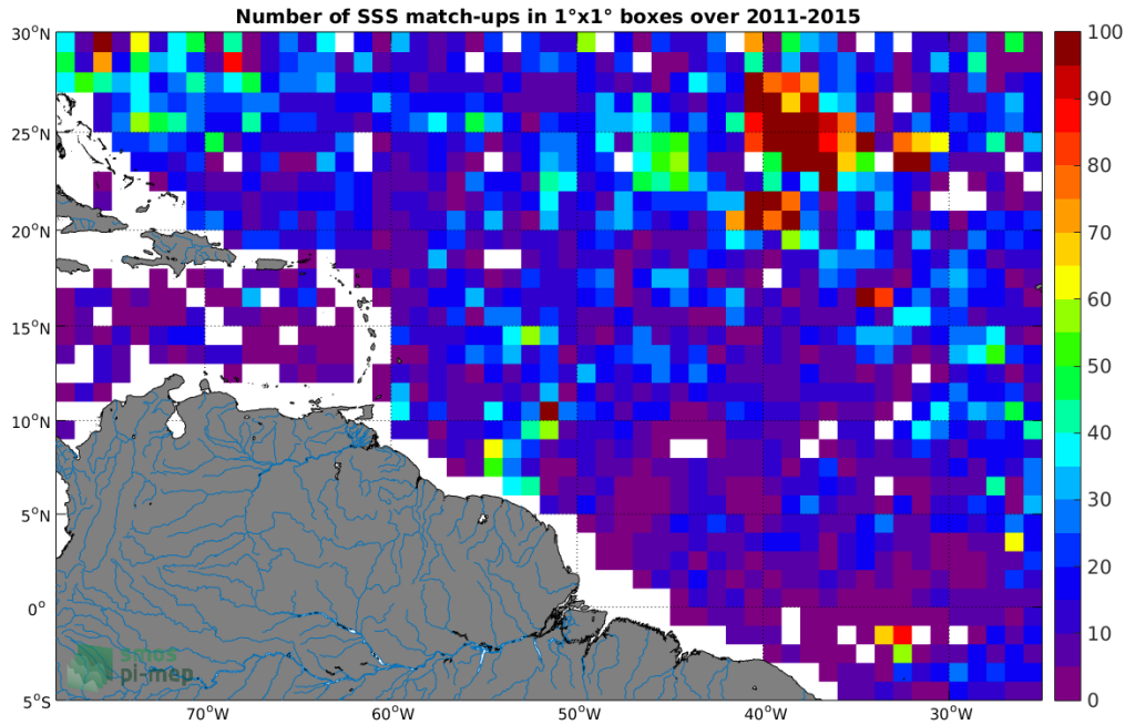
Figure 4: Number of SSS match-ups between Argo SSS and the Aquarius SSS L2-AVERAGED OR v5 (NASA-GSFC) SSS product for the Amazon and Orinoco river plumes Pi-MEP region over 1^\circ \times 1^\circ boxes and for the full satellite product period.
