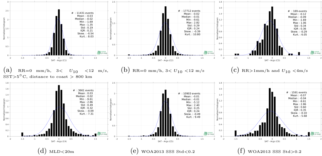
Figure 13: Normalized histogram of \Delta\text{SSS} (Aquarius SSS L2-AVERAGED OR v5 (NASA-GSFC) - Argo) for 6 different subdatasets corresponding to: RR=0 mm/h, 3 < U_{10} < 12 m/s, SST>5°C, distance to coast > 800 km (a), RR=0 mm/h, 3 < U_{10} < 12 m/s (b), RR>1mm/h and U_{10} < 4 m/s (c), MLD<20m (d), WOA2013 SSS Std<0.2 (e), WOA2013 SSS Std>0.2 (f).
