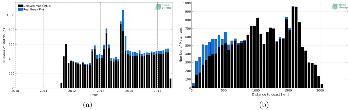
Figure 1: Number of match-ups between Argo and Aquarius SSS L2-AVERAGED OR v5 (NASA-GSFC) SSS as a function of time (a) and as function of the distance to coast (b) over the Amazon and Orinoco river plumes Pi-MEP region and for the full satellite product period.
