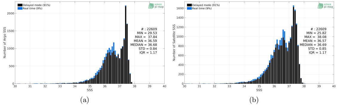
Figure 2: Histograms of SSS from Argo (a) and Aquarius SSS L2-AVERAGED OR v5 (NASA-GSFC) (b) considering all match-up pairs per bins of 0.1 over the Amazon and Orinoco river plumes Pi-MEP region and for the full satellite product period.
