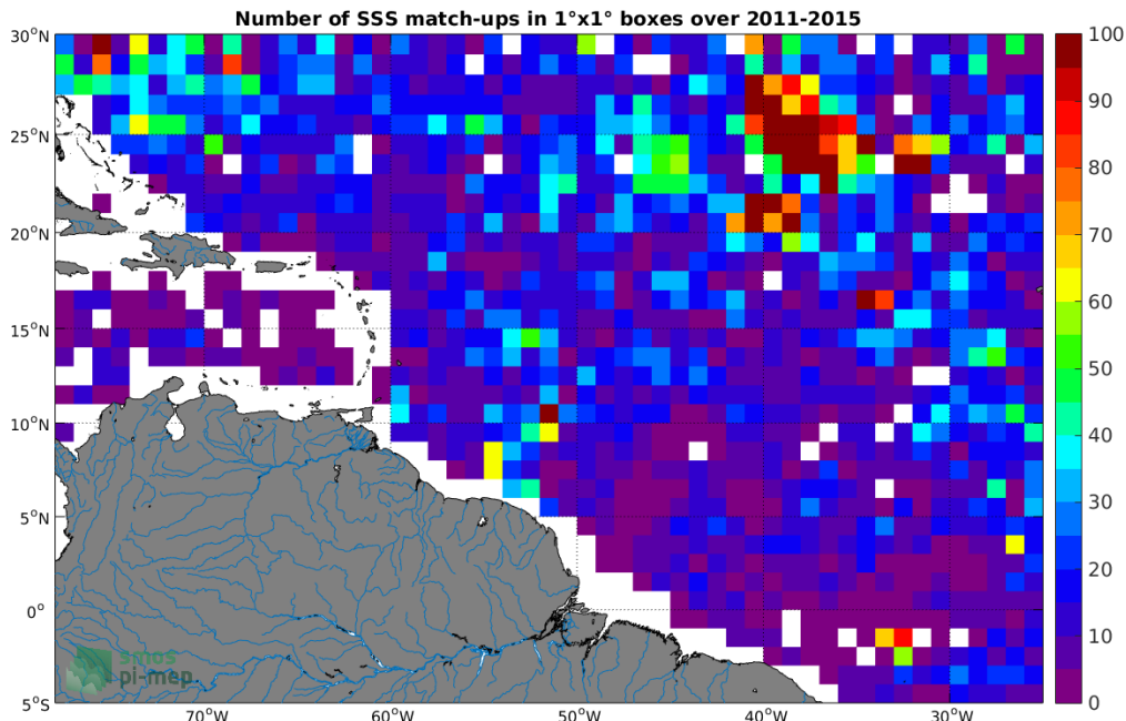
Figure 4: Number of SSS match-ups between Argo SSS and the Aquarius SSS L2-AVERAGED CAP v5 (JPL) SSS product for the Amazon and Orinoco river plumes Pi-MEP region over 1^\circ \times 1^\circ boxes and for the full satellite product period.
