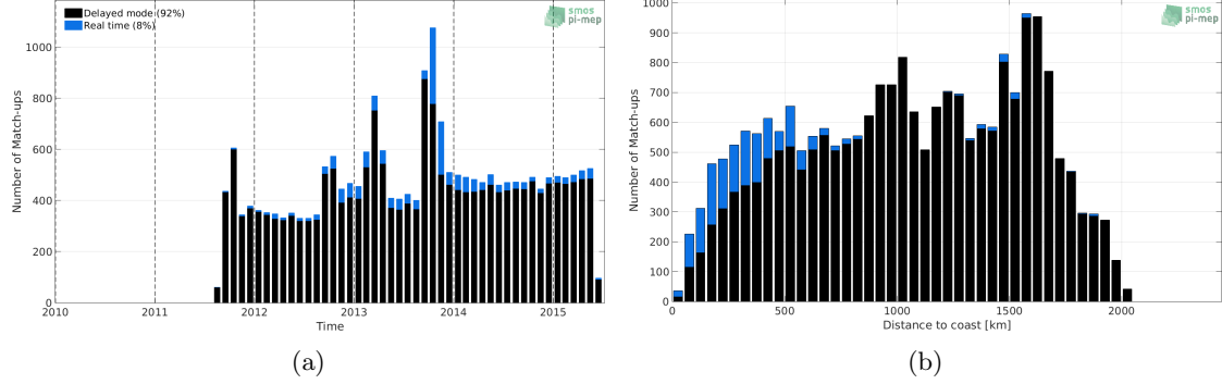
Figure 1: Number of match-ups between Argo and Aquarius SSS L2-AVERAGED CAP v5 (JPL) SSS as a function of time (a) and as function of the distance to coast (b) over the Amazon and Orinoco river plumes Pi-MEP region and for the full satellite product period.
