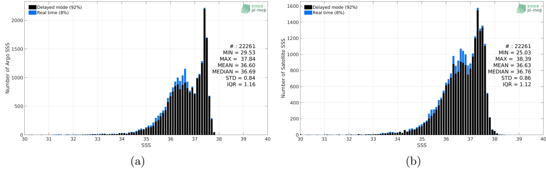
Figure 2: Histograms of SSS from Argo (a) and Aquarius SSS L2-AVERAGED CAP v5 (JPL) (b) considering all match-up pairs per bins of 0.1 over the Amazon and Orinoco river plumes Pi-MEP region and for the full satellite product period.
