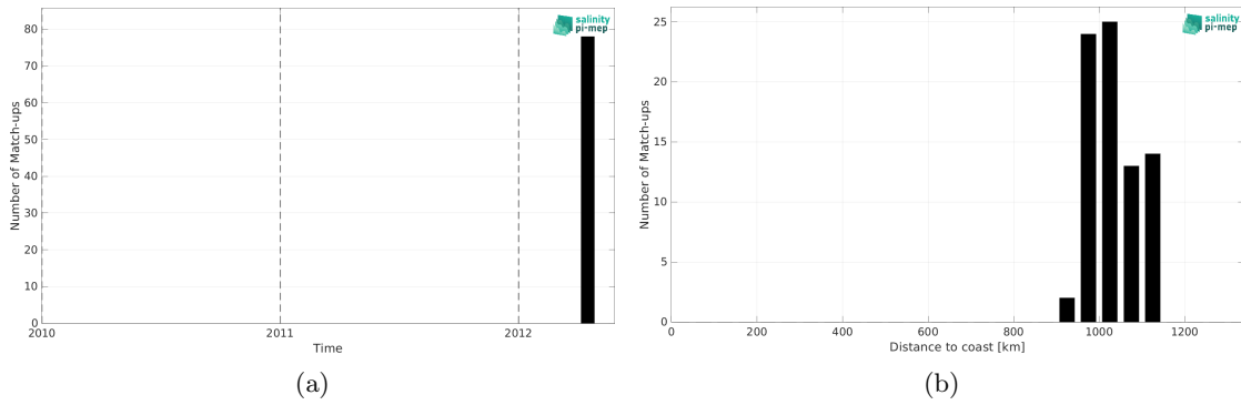
Figure 2: Number of match-ups between TSG (Polarstern) and Aquarius SSS L2 OR v5 (NASA-GSFC) SSS as a function of time (a) and as function of the distance to coast (b) over the Amazon and Orinoco river plumes Pi-MEP region and for the full satellite product period.
