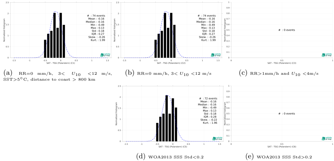
Figure 15: Normalized histogram of \Delta SSS (Aquarius SSS L2 OR v5 (NASA-GSFC) - TSG (Polarstern)) for 5 different subdatasets corresponding to: RR=0 mm/h, 3 < U_{10} < 12 m/s, SST >5^{\circ} C, distance to coast > 800 km (a), RR=0 mm/h, 3 < U_{10} < 12 m/s (b), RR >1 mm/h and U_{10} < 4 m/s (c), WOA2013 SSS Std <0.2 (d), WOA2013 SSS Std >0.2 (e).
