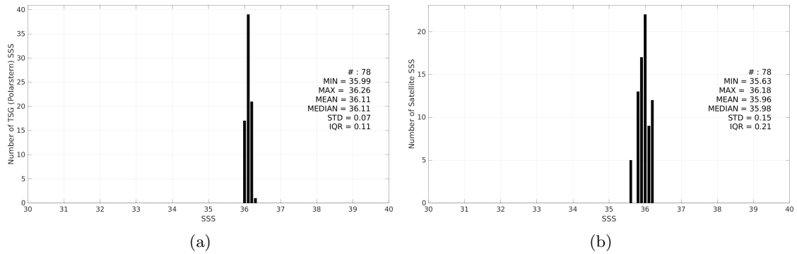
Figure 3: Histograms of SSS from TSG (Polarstern) (a) and Aquarius SSS L2 OR v5 (NASA-GSFC) (b) considering all match-up pairs per bins of 0.1 over the Amazon and Orinoco river plumes Pi-MEP region and for the full satellite product period.
