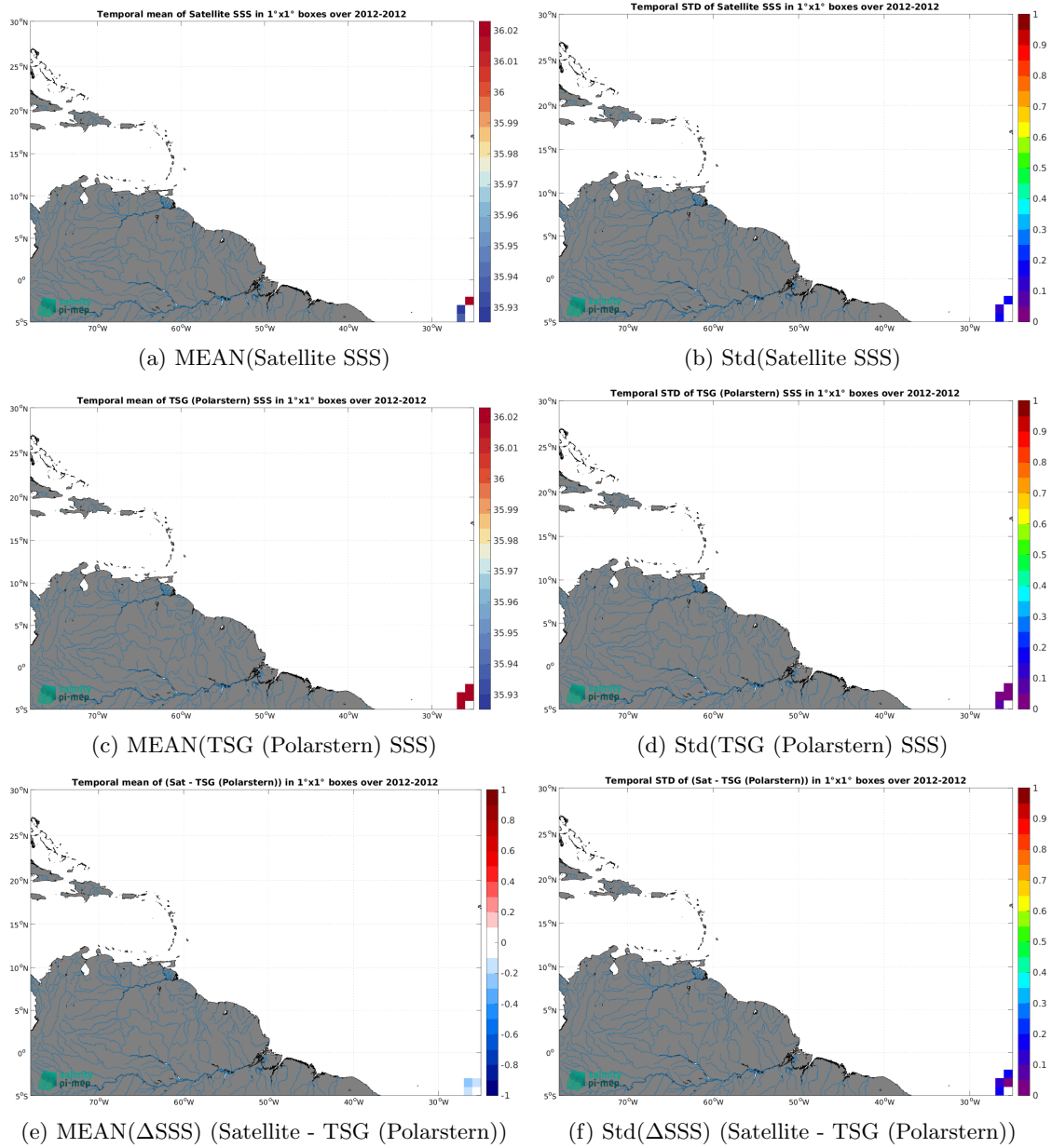
Figure 7: Temporal mean (left) and Std (right) of SSS from Aquarius SSS L2 OR v5 (NASA-GSFC) (top), TSG (Polarstern) (middle), and of \Delta SSS (Satellite - TSG (Polarstern)). Only match-up pairs are used to generate these maps.
