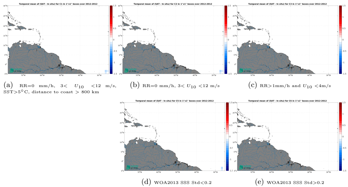
Figure 14: Temporal mean gridded over spatial boxes of size 1^\circ \times 1^\circ of \Delta SSS (Aquarius SSS L2 OR v5 (NASA-GSFC) - TSG (Polarstern)) for 5 different subdatasets corresponding to:RR=0 mm/h, 3 < U_{10} < 12 m/s, SST > 5°C, distance to coast > 800 km (a), RR=0 mm/h, 3 < U_{10} < 12 m/s (b), RR > 1mm/h and U_{10} < 4 m/s (c), WOA2013 SSS Std < 0.2 (d), WOA2013 SSS Std > 0.2 (e).
