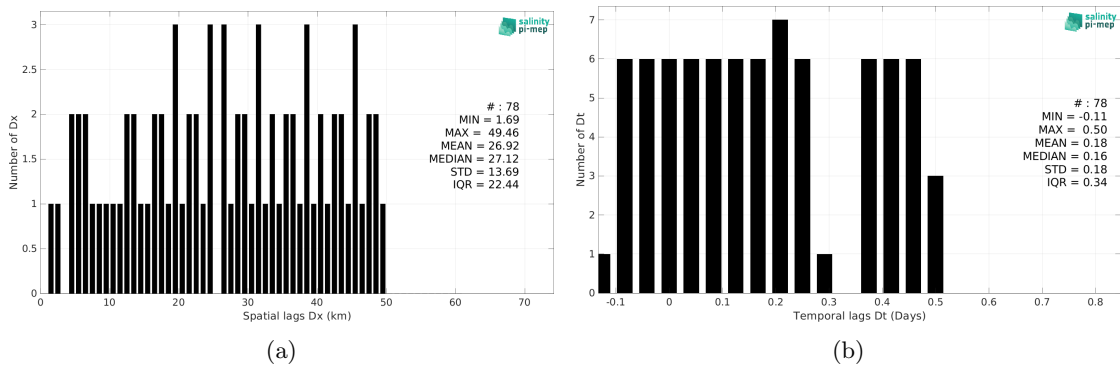
Figure 6: Histograms of the spatial (a) and temporal (b) lags between the location/time of the TSG (Polarstern) measurement and the date of the corresponding Aquarius SSS L2 OR v5 (NASA-GSFC) SSS pixel.
