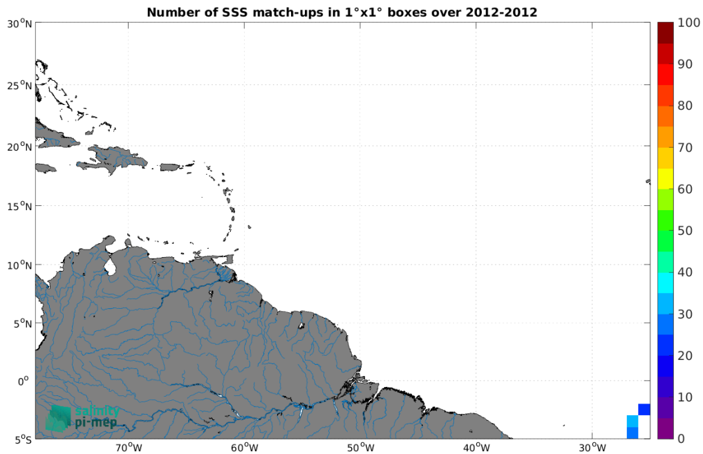
Figure 5: Number of SSS match-ups between TSG (Polarstern) SSS and the Aquarius SSS L2 OR v5 (NASA-GSFC) SSS product for the Amazon and Orinoco river plumes Pi-MEP region over 1^\circ \times 1^\circ boxes and for the full satellite product period.
