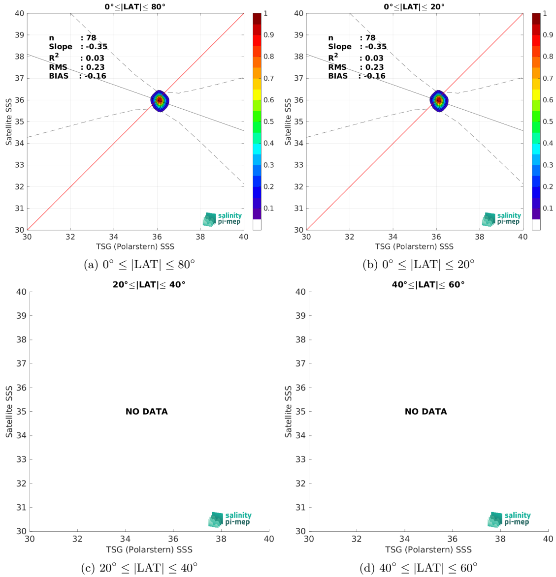
Figure 10: Contour maps of the concentration of Aquarius SSS L2 OR v5 (NASA-GSFC) SSS (y-axis) versus TSG (Polarstern) SSS (x-axis) at match-up pairs for different latitude bands. For each plot, the red line shows x=y . The black thin and dashed lines indicate a linear fit through the data cloud and the \pm 95\% confidence levels, respectively. The number match-up pairs n , the slope and R^2 coefficient of the linear fit, the root mean square (RMS) and the mean bias between satellite and in situ data are indicated for each latitude band in each plots.
