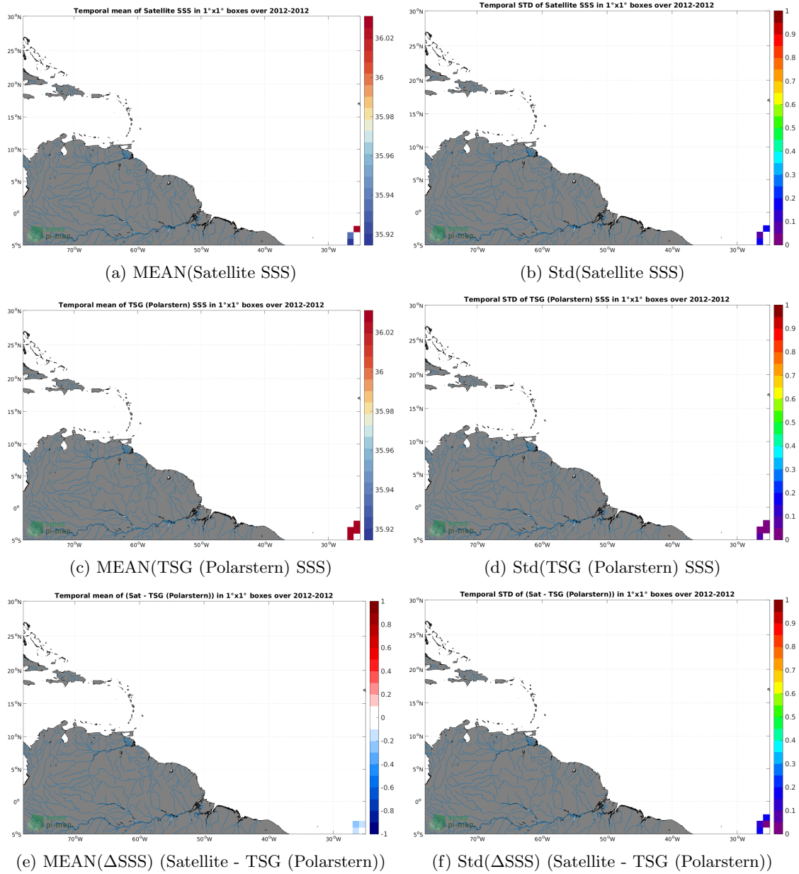
Figure 6: Temporal mean (left) and Std (right) of SSS from Aquarius SSS L2 OR v5 (NASA-GSFC) (top), TSG (Polarstern) (middle), and of \Delta SSS (Satellite - TSG (Polarstern)). Only match-up pairs are used to generate these maps.
