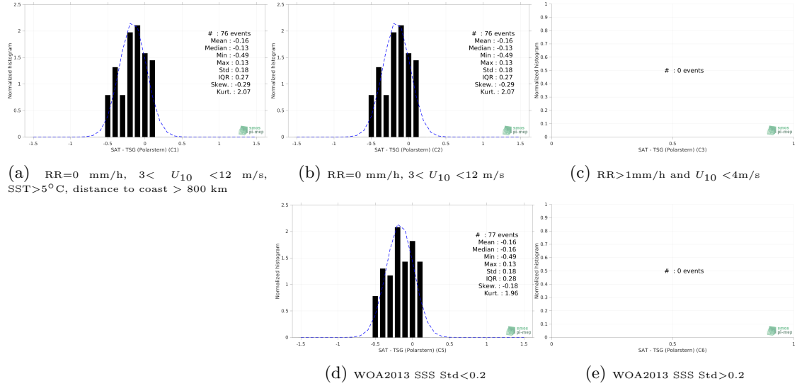
Figure 13: Normalized histogram of \Delta SSS (Aquarius SSS L2 OR v5 (NASA-GSFC) - TSG (Polarstern)) for 5 different subdatasets corresponding to: RR=0 mm/h, 3 < U_{10} < 12 m/s, SST>5°C, distance to coast > 800 km (a), RR=0 mm/h, 3 < U_{10} < 12 m/s (b), RR>1mm/h and U_{10} < 4 m/s (c), WOA2013 SSS Std<0.2 (d), WOA2013 SSS Std>0.2 (e).
