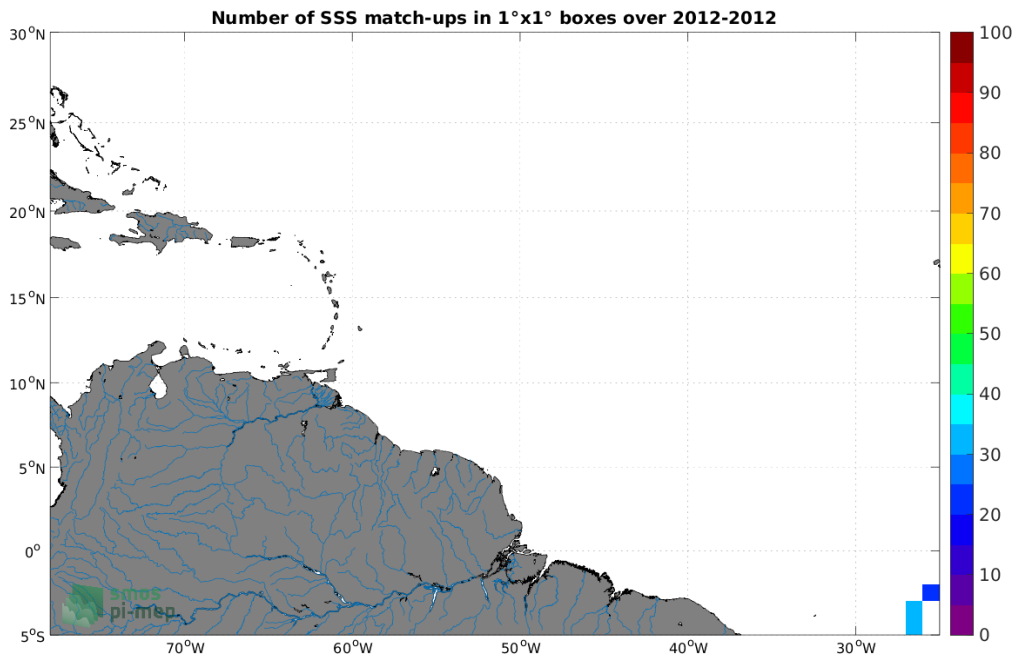
Figure 4: Number of SSS match-ups between TSG (Polarstern) SSS and the Aquarius SSS L2 OR v5 (NASA-GSFC) SSS product for the Amazon and Orinoco river plumes Pi-MEP region over 1°x1° boxes and for the full satellite product period.
