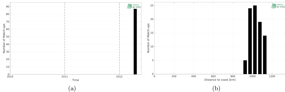
Figure 1: Number of match-ups between TSG (Polarstern) and Aquarius SSS L2 OR v5 (NASA-GSFC) SSS as a function of time (a) and as function of the distance to coast (b) over the Amazon and Orinoco river plumes Pi-MEP region and for the full satellite product period.
