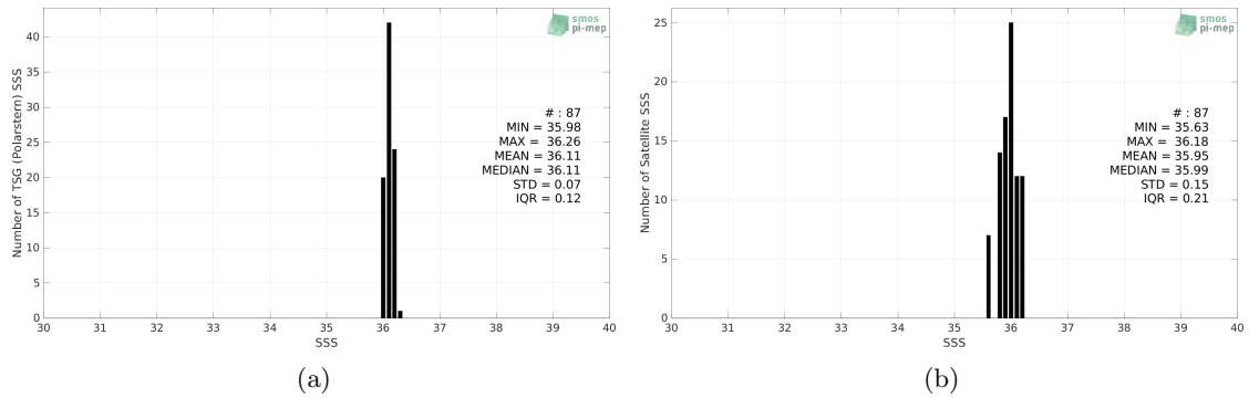
Figure 2: Histograms of SSS from TSG (Polarstern) (a) and Aquarius SSS L2 OR v5 (NASA-GSFC) (b) considering all match-up pairs per bins of 0.1 over the Amazon and Orinoco river plumes Pi-MEP region and for the full satellite product period.
