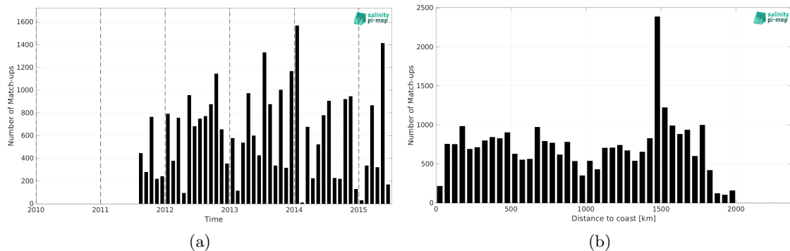
Figure 2: Number of match-ups between TSG (LEGOS-DM) and Aquarius SSS L2 OR v5 (NASA-GSFC) SSS as a function of time (a) and as function of the distance to coast (b) over the Amazon and Orinoco river plumes Pi-MEP region and for the full satellite product period.
