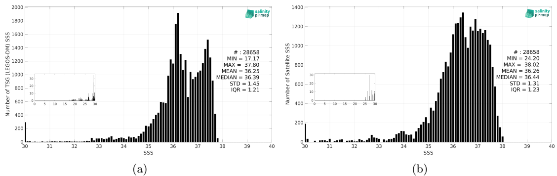
Figure 3: Histograms of SSS from TSG (LEGOS-DM) (a) and Aquarius SSS L2 OR v5 (NASA-GSFC) (b) considering all match-up pairs per bins of 0.1 over the Amazon and Orinoco river plumes Pi-MEP region and for the full satellite product period.
