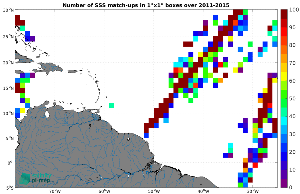
Figure 5: Number of SSS match-ups between TSG (LEGOS-DM) SSS and the Aquarius SSS L2 OR v5 (NASA-GSFC) SSS product for the Amazon and Orinoco river plumes Pi-MEP region over 1^\circ \times 1^\circ boxes and for the full satellite product period.
