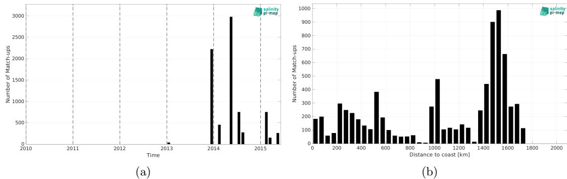
Figure 2: Number of match-ups between TSG (GOSUD-Sailing-ship) and Aquarius SSS L2 OR v5 (NASA-GSFC) SSS as a function of time (a) and as function of the distance to coast (b) over the Amazon and Orinoco river plumes Pi-MEP region and for the full satellite product period.
