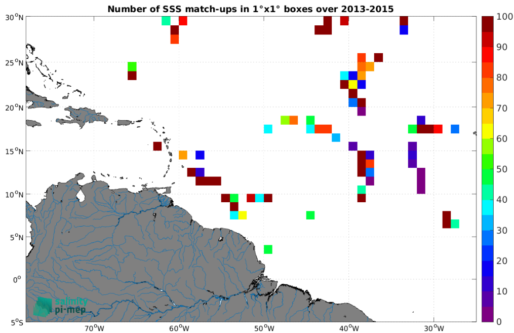
Figure 5: Number of SSS match-ups between TSG (GOSUD-Sailing-ship) SSS and the Aquarius SSS L2 OR v5 (NASA-GSFC) SSS product for the Amazon and Orinoco river plumes Pi-MEP region over 1^\circ \times 1^\circ boxes and for the full satellite product period.
