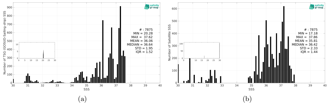
Figure 3: Histograms of SSS from TSG (GOSUD-Sailing-ship) (a) and Aquarius SSS L2 OR v5 (NASA-GSFC) (b) considering all match-up pairs per bins of 0.1 over the Amazon and Orinoco river plumes Pi-MEP region and for the full satellite product period.
