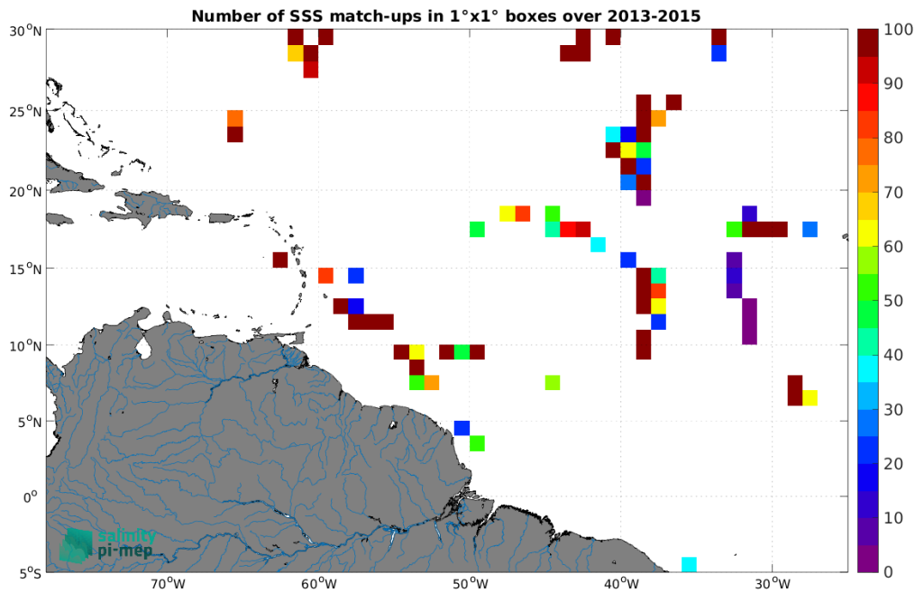
Figure 4: Number of SSS match-ups between TSG (GOSUD-Sailing-ship) SSS and the Aquarius SSS L2 OR v5 (NASA-GSFC) SSS product for the Amazon and Orinoco river plumes Pi-MEP region over 1^\circ \times 1^\circ boxes and for the full satellite product period.
