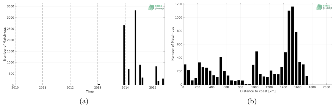
Figure 1: Number of match-ups between TSG (GOSUD-Sailing-ship) and Aquarius SSS L2 OR v5 (NASA-GSFC) SSS as a function of time (a) and as function of the distance to coast (b) over the Amazon and Orinoco river plumes Pi-MEP region and for the full satellite product period.
