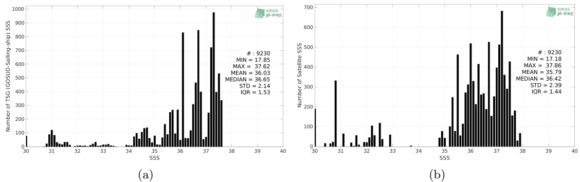
Figure 2: Histograms of SSS from TSG (GOSUD-Sailing-ship) (a) and Aquarius SSS L2 OR v5 (NASA-GSFC) (b) considering all match-up pairs per bins of 0.1 over the Amazon and Orinoco river plumes Pi-MEP region and for the full satellite product period.
