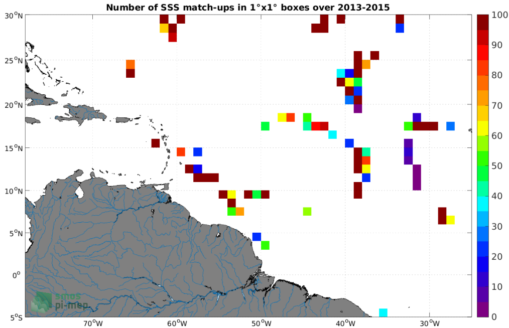
Figure 4: Number of SSS match-ups between TSG (GOSUD-Sailing-ship) SSS and the Aquarius SSS L2 OR v5 (NASA-GSFC) SSS product for the Amazon and Orinoco river plumes Pi-MEP region over 1^{\circ} \times 1^{\circ} boxes and for the full satellite product period.
